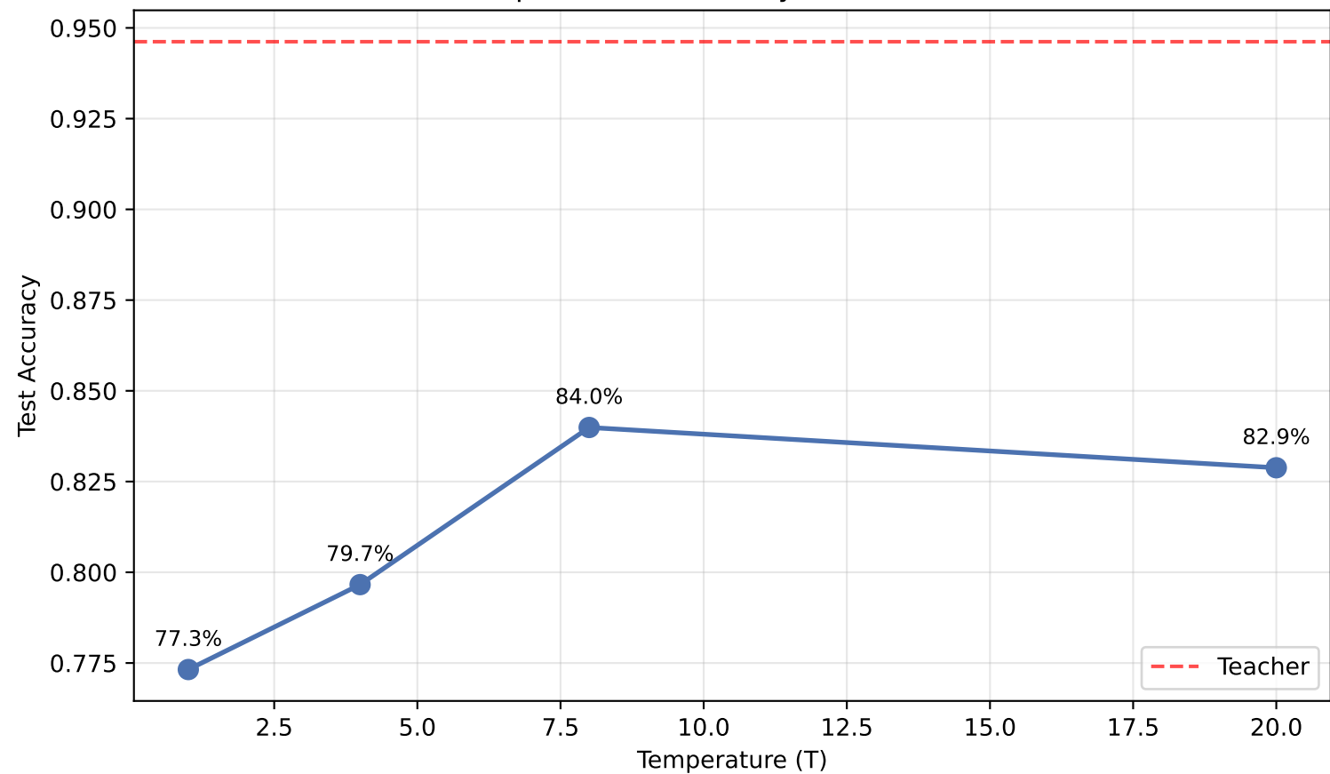
Scenario C: Temperature Sensitivity — ResNet-34 → ResNet-18
