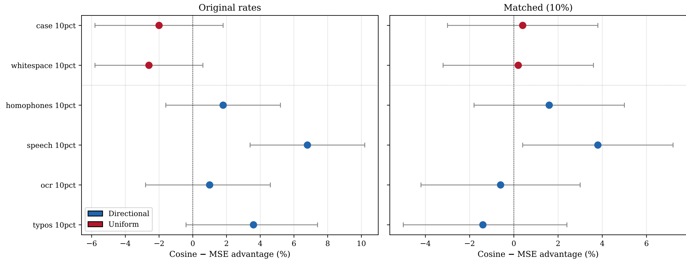
Cosine vs MSE Advantage by Perturbation Type and Rate Condition
