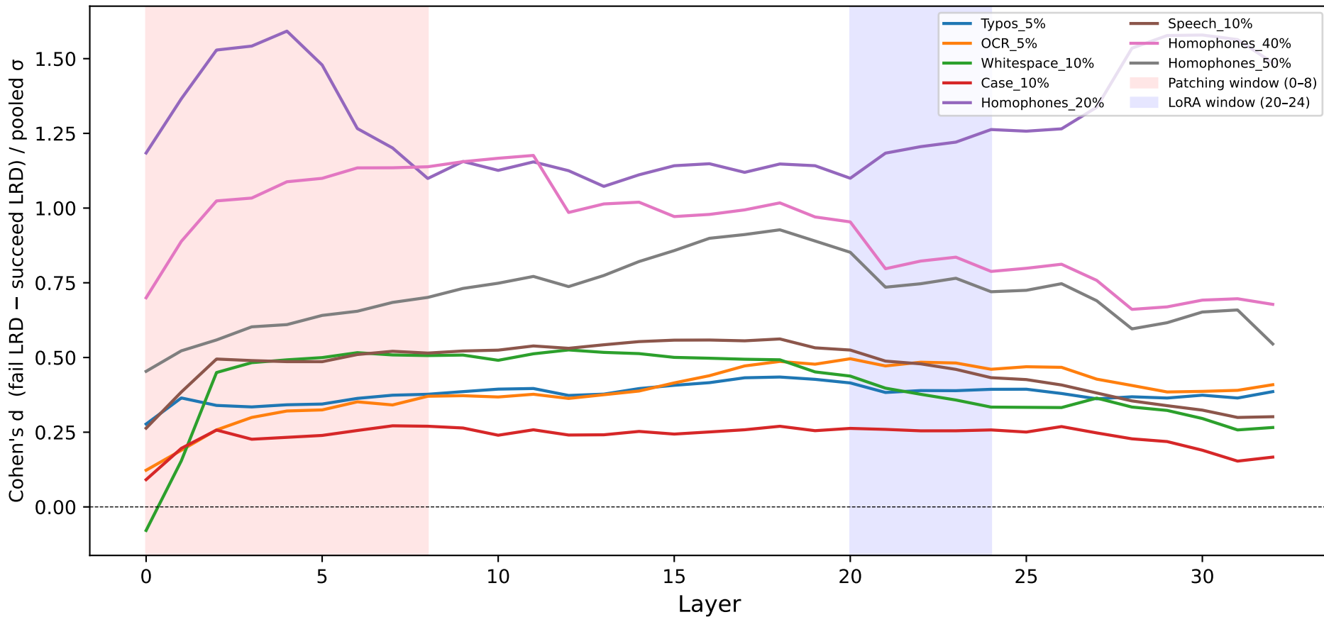
Per-Layer Cohen's d Profile — Mistral / GSM8K
