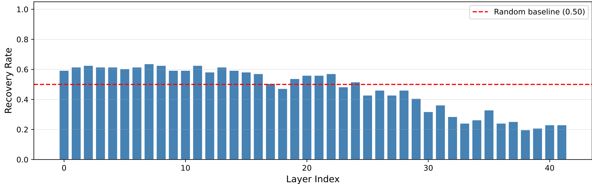
Activation Patching — GSM8K typos @ 0.05 (n=91 pairs)
