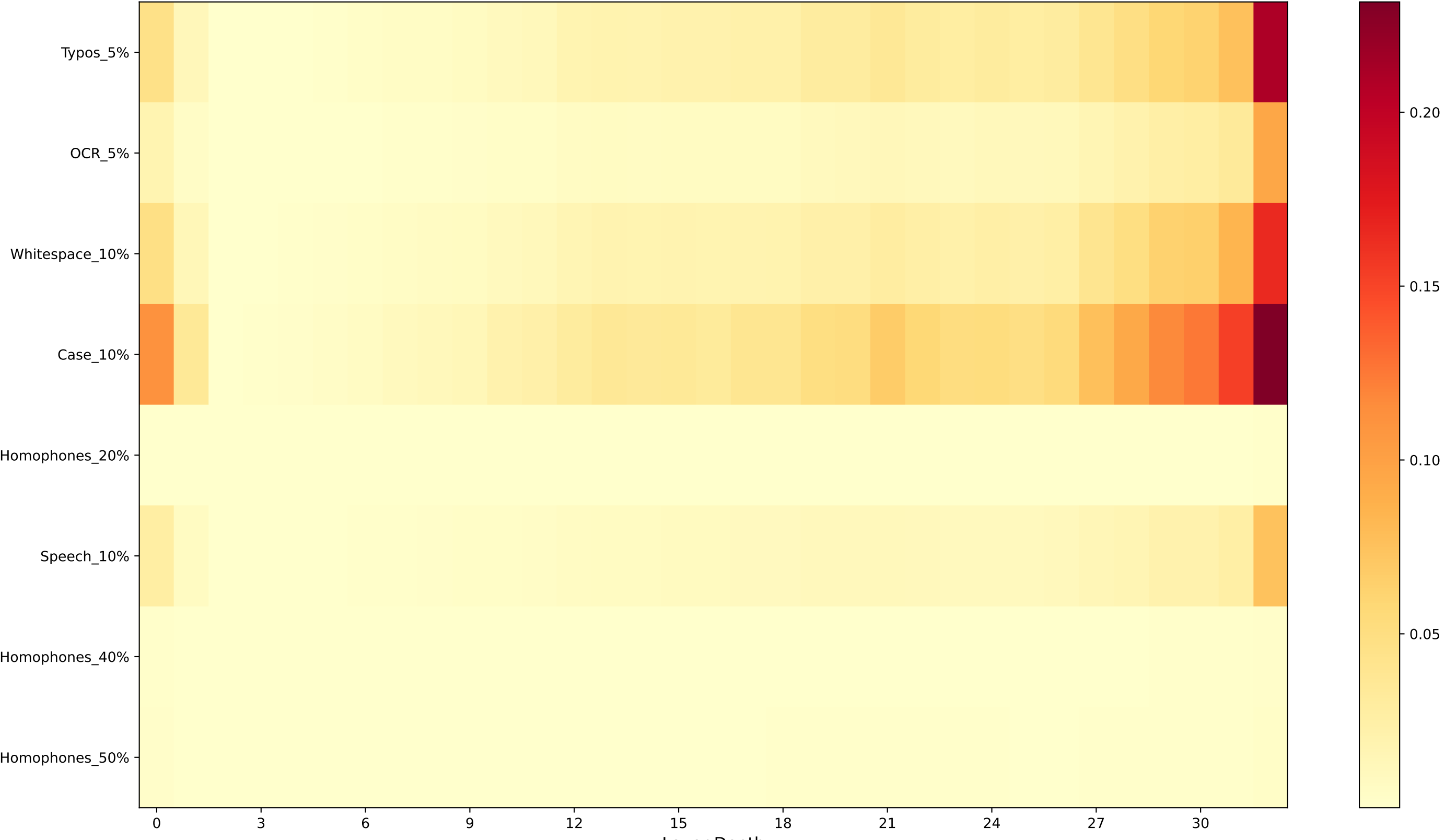
LRD Heatmap (Perturbation \times Layer) — BBL
