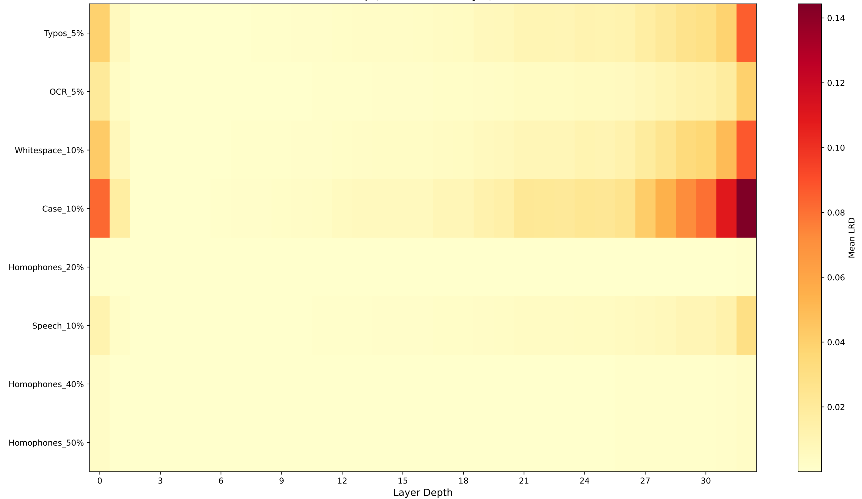
LRD Heatmap (Perturbation × Layer) — GSM8K
