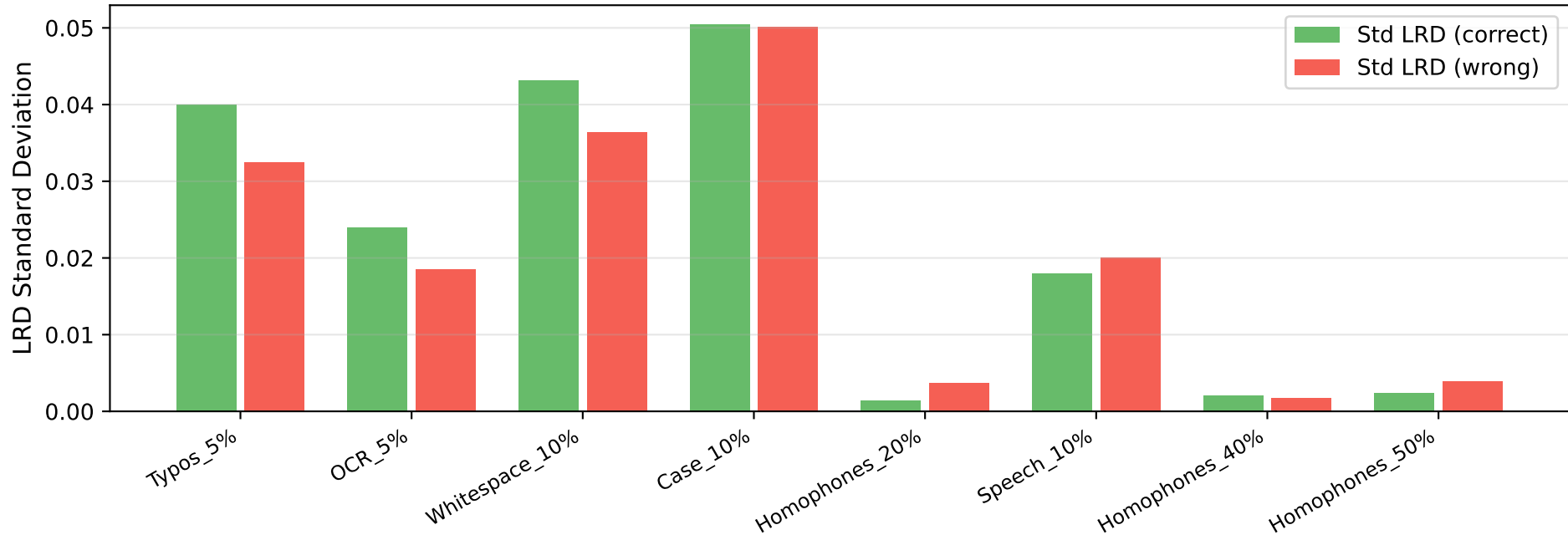
Within-Group LRD Variance by Perturbation — MMLU Levene p=0.0000 (not supported)
