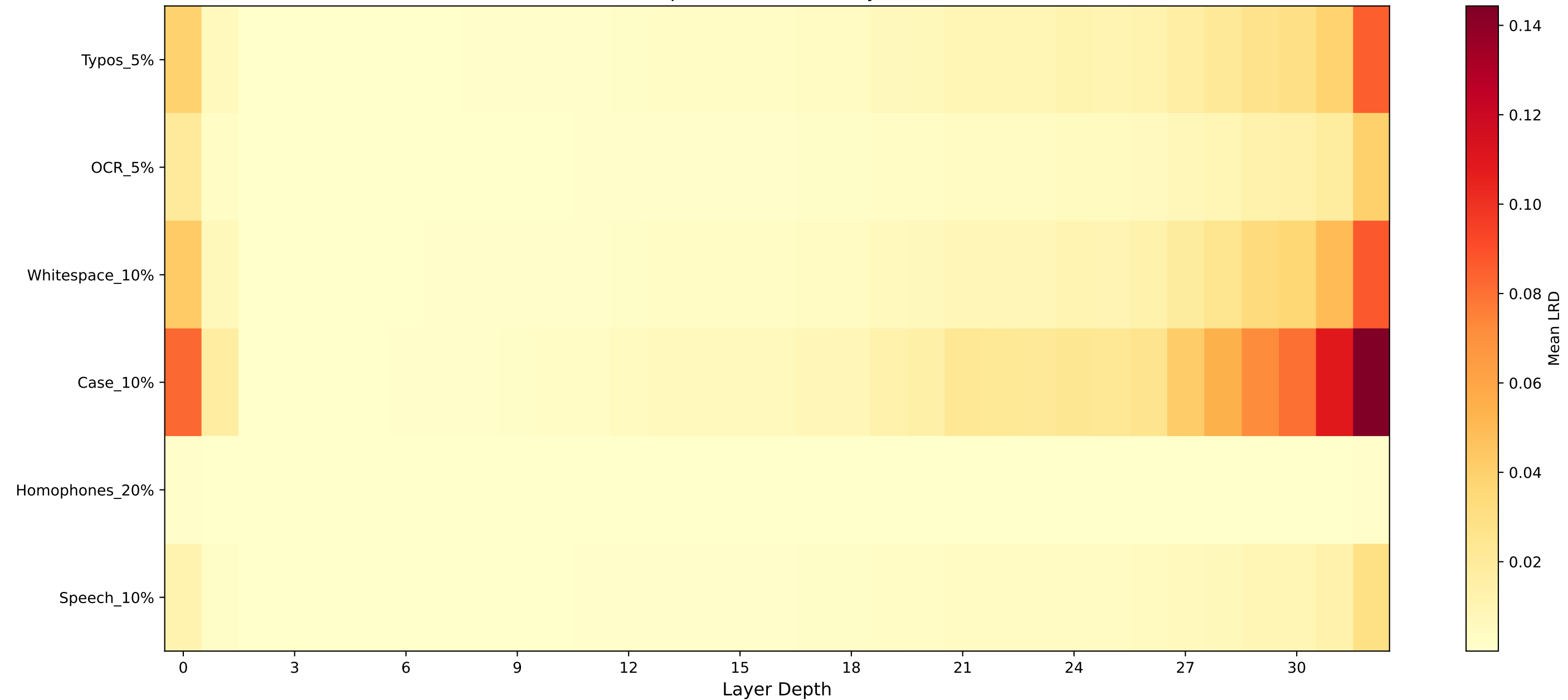
LRD Heatmap (Perturbation × Layer) — GSM8K
