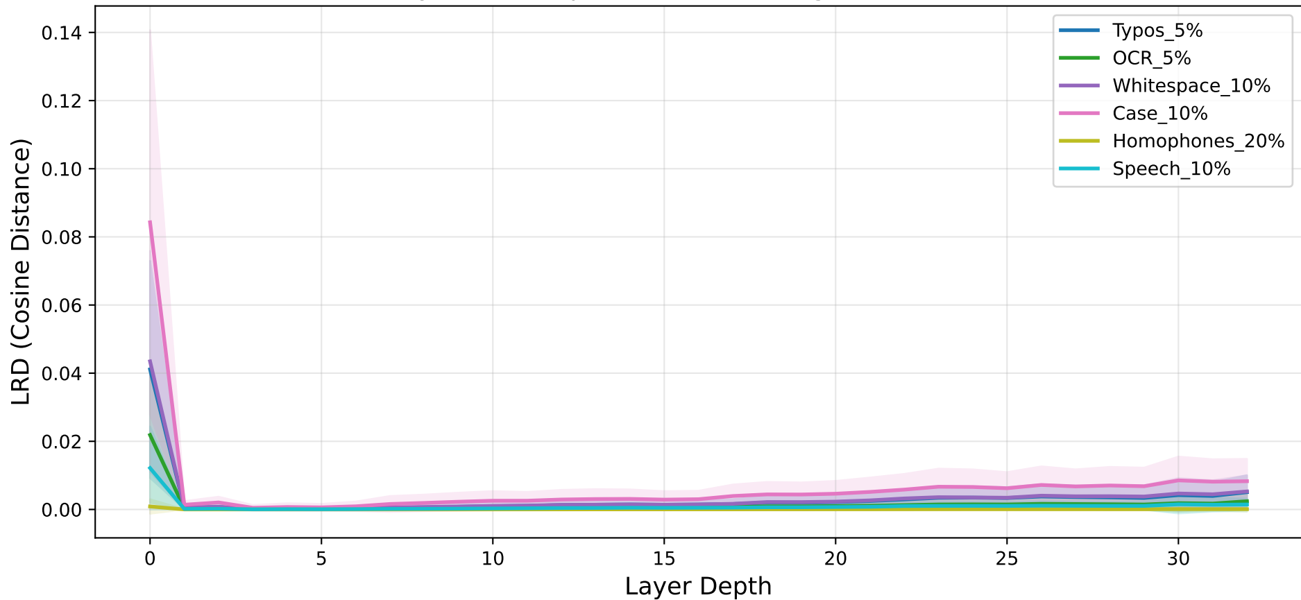
Layer-Wise Representation Divergence — MMLU
