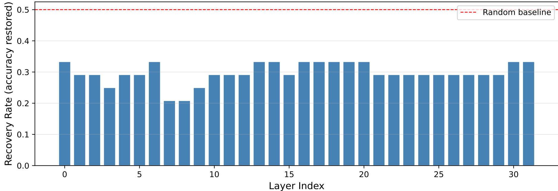
Activation Patching: Which layer causally mediates failure? MMLU — typos @ 0.05
