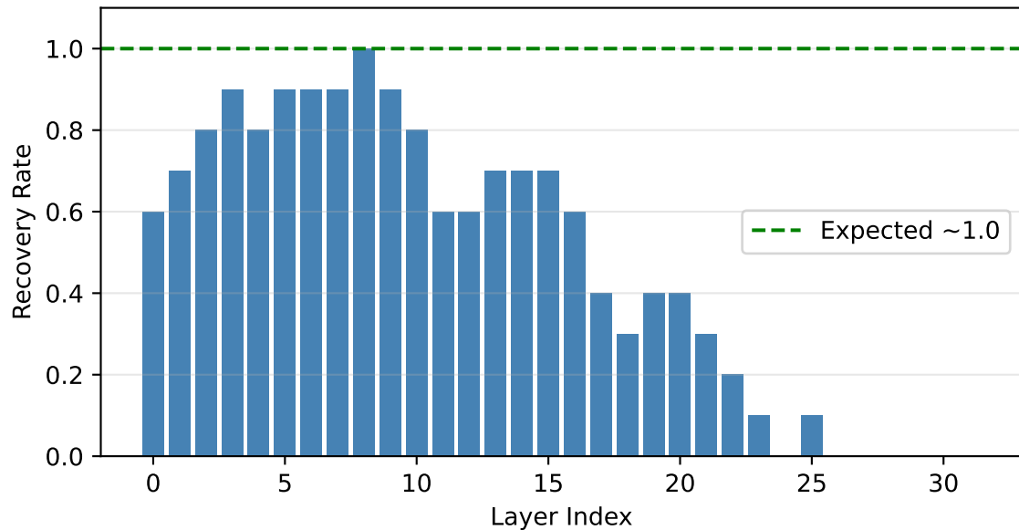
Positive Control: Identity Patch (should be ~100%)
