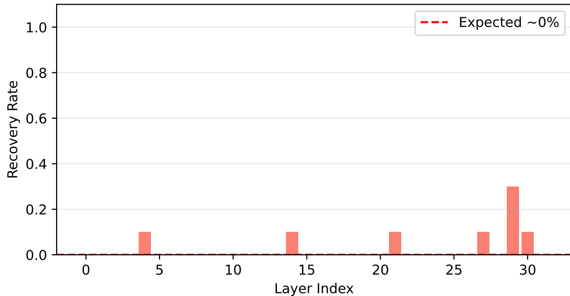
Negative Control: Random Noise Patch (should be ~0%)
