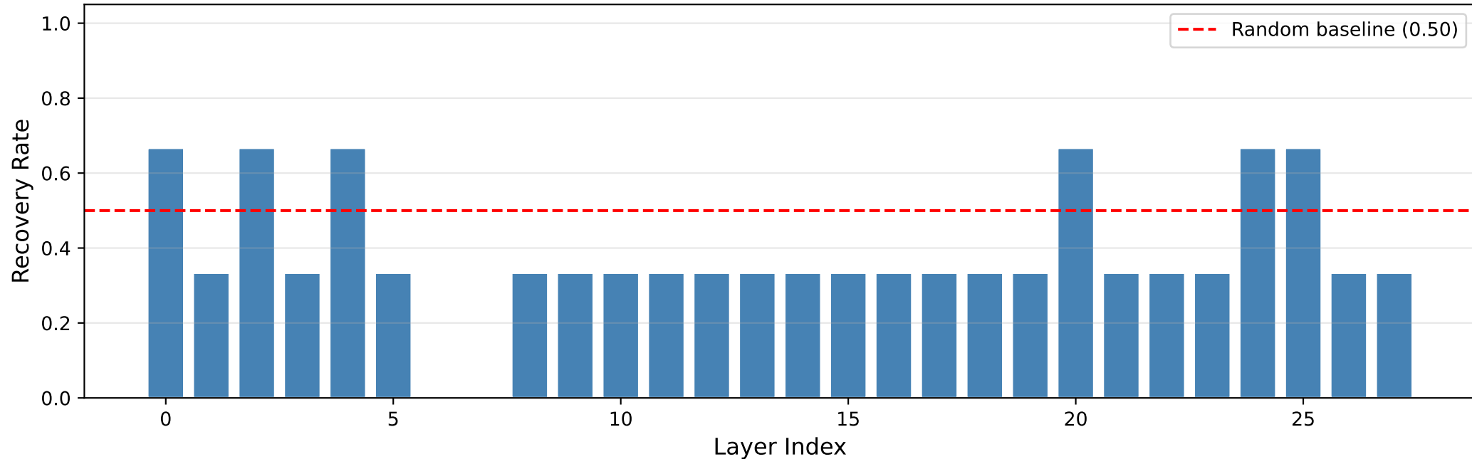
Activation Patching — GSM8K typos @ 0.05 (n=3 pairs)
