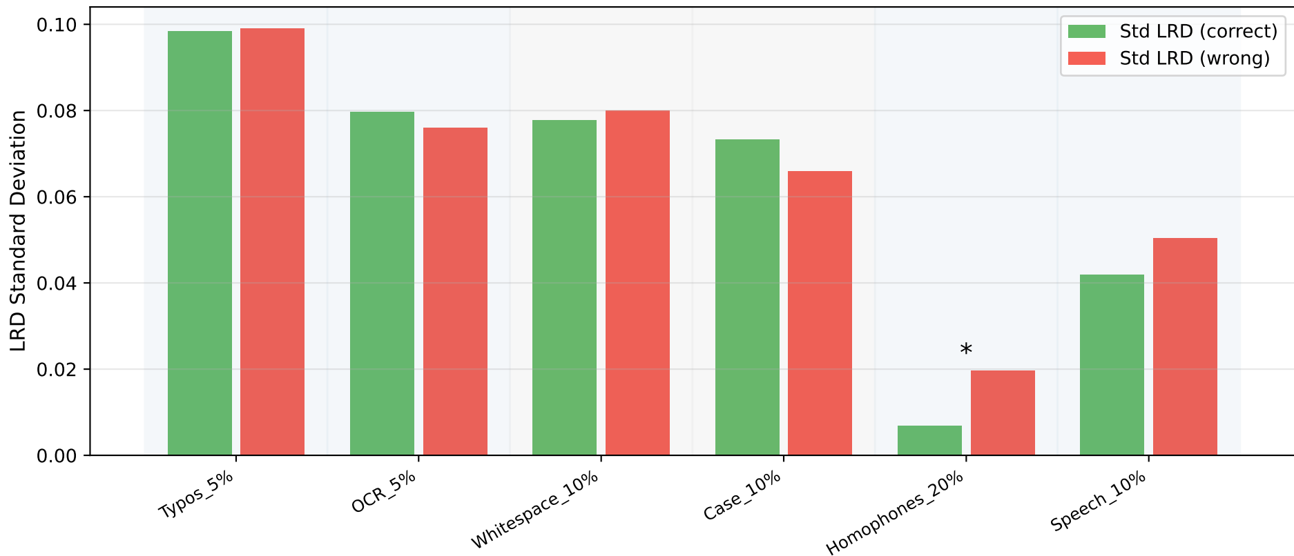
Per-Perturbation Wrong vs Correct LRD Variance — GSM8K Blue shading = directional class | * = Levene p<0.05 with wrong_std > correct_std Taxonomy not supported (1/4 directional types confirmed)
