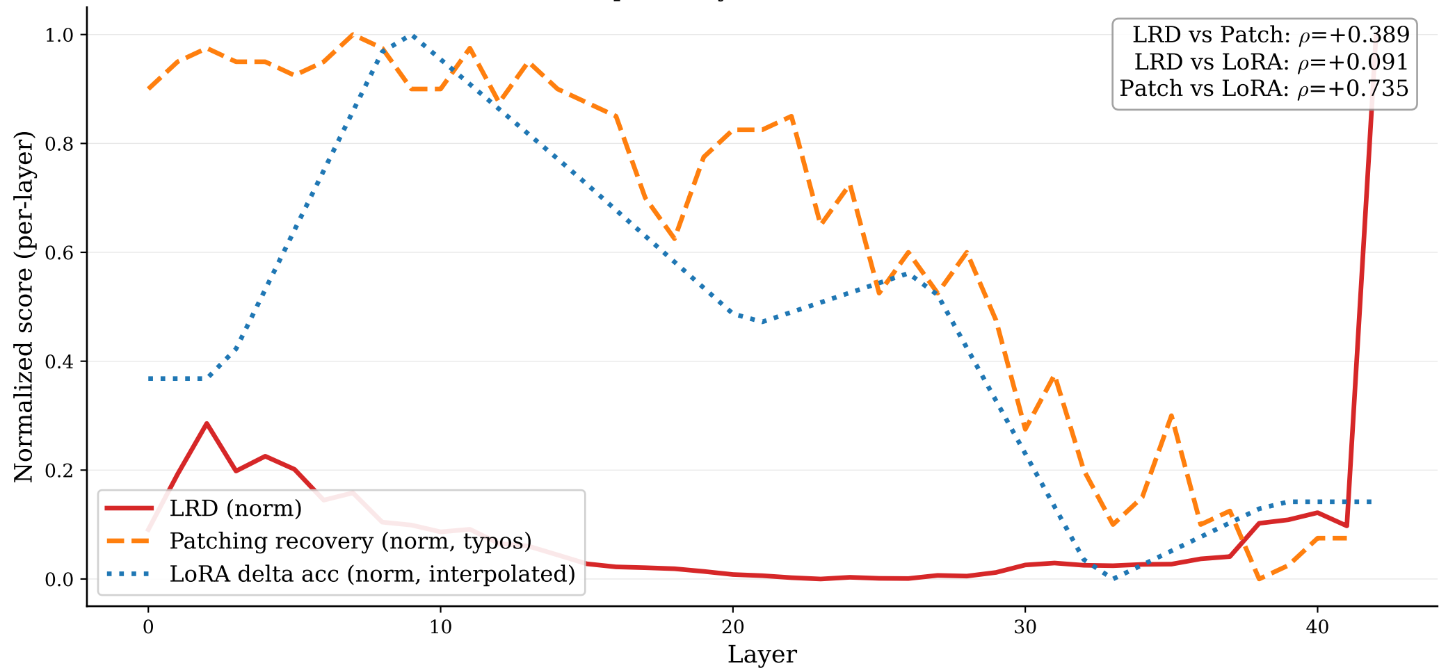
Three-Map Overlay - Gemma-2-9B / GSM8K
