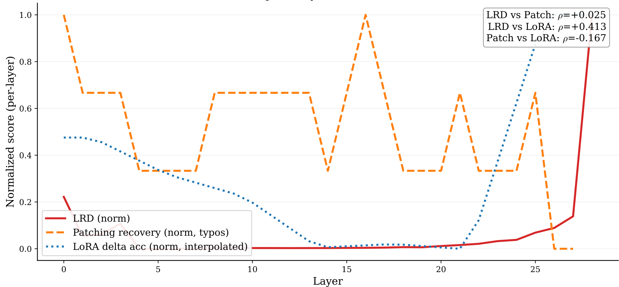
Three-Map Overlay - Qwen2.5-7B / GSM8K
