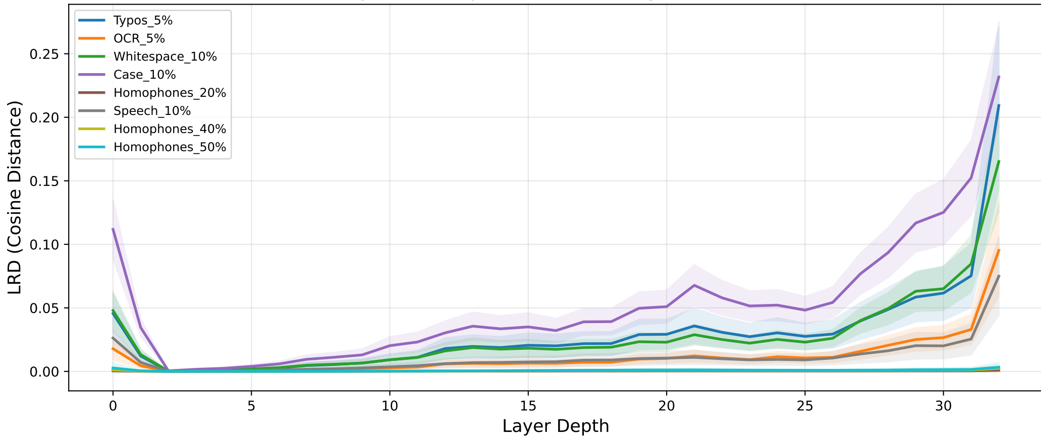
Layer-Wise Representation Divergence — BBH
