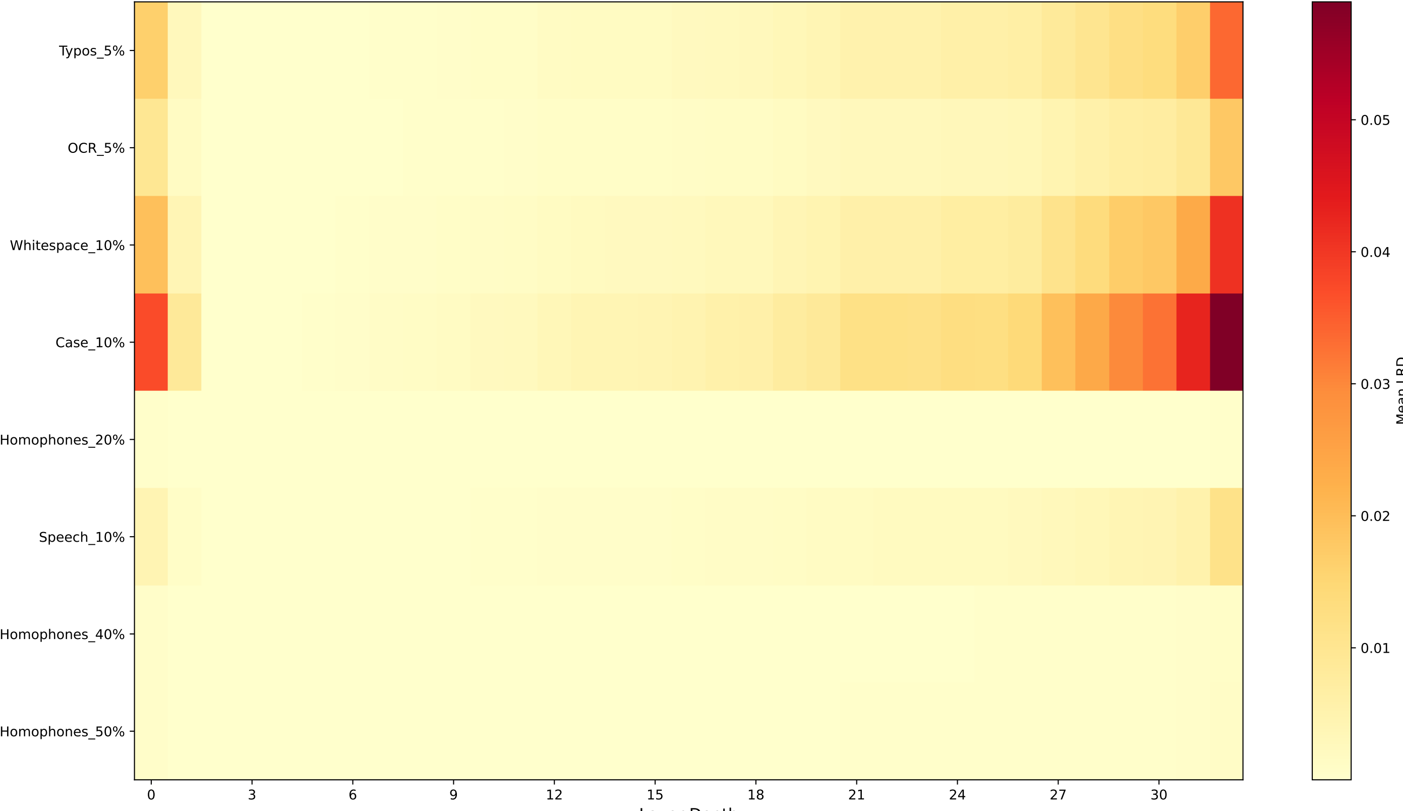
LRD Heatmap (Perturbation \times Layer) — MMLU
