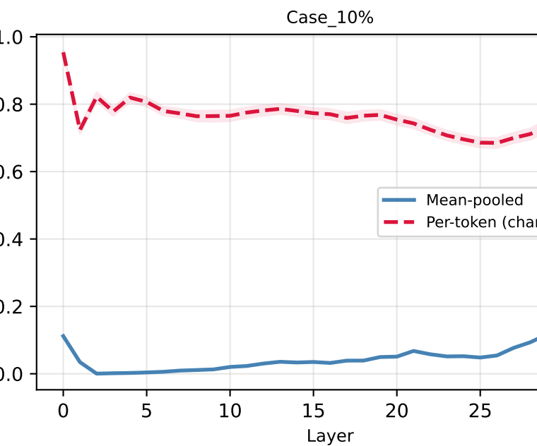
Mean-Pooled vs Per-Token LRD — BBH (Per-token = changed positions only; mean-pooled is a lower bound)
