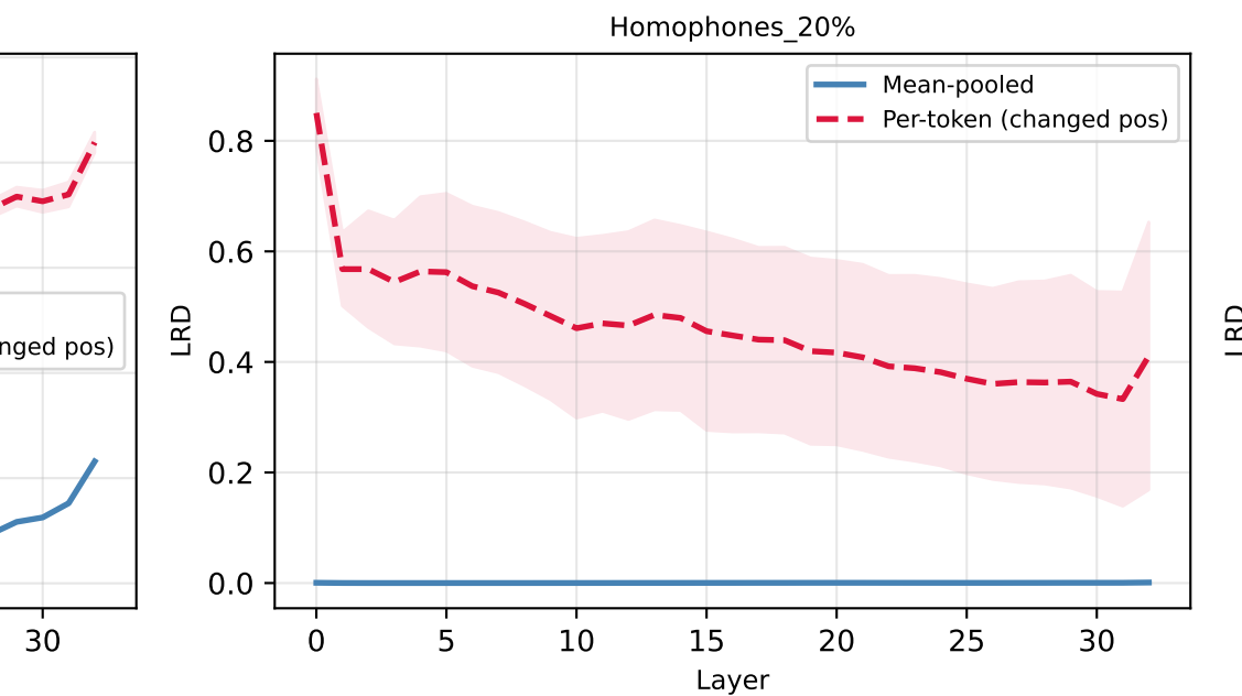
Mean-Pooled vs Per-Token LRD — BBH (Per-token = changed positions only; mean-pooled is a lower bound)
