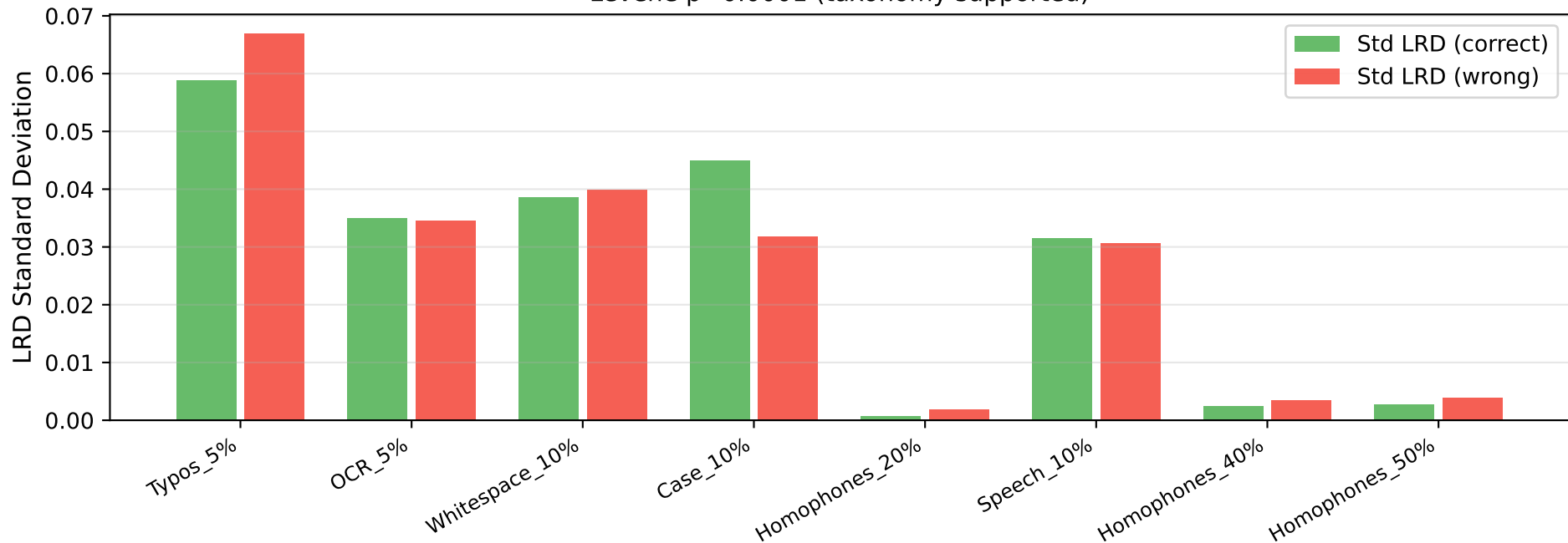
Within-Group LRD Variance by Perturbation — BBH Levene p=0.0001 (taxonomy supported)
