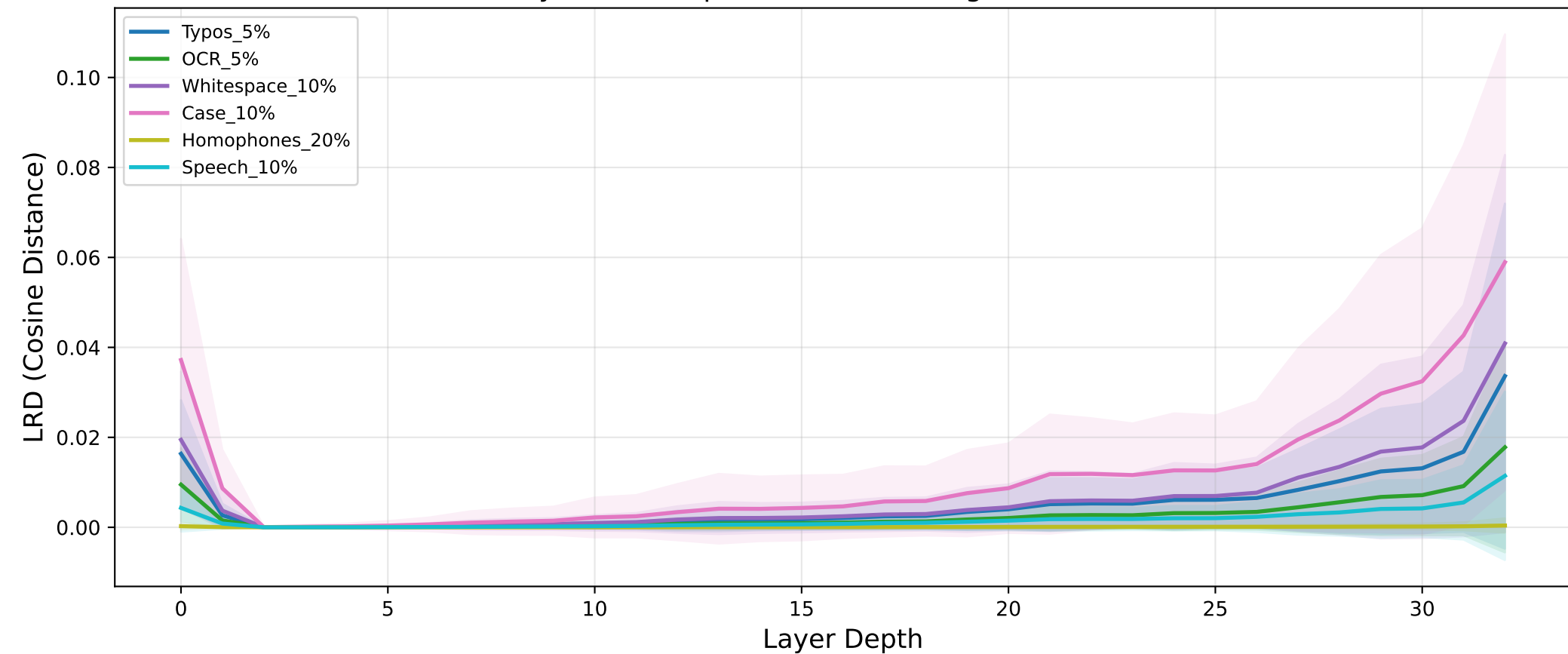
Layer-Wise Representation Divergence — MMLU
