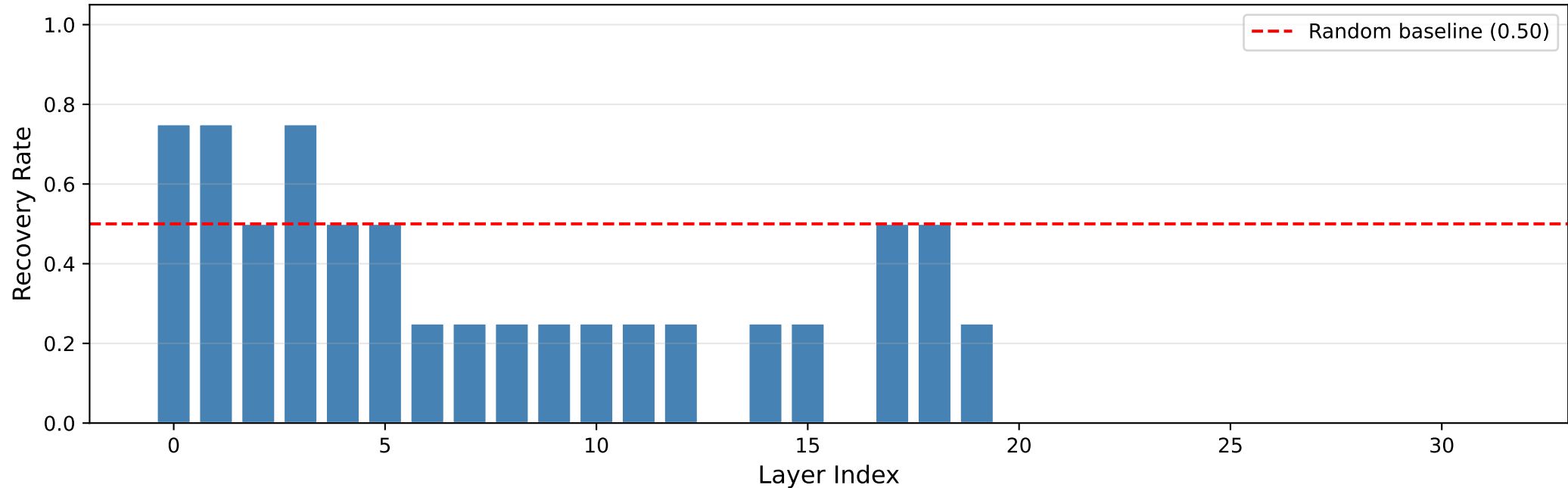
Activation Patching — GSM8K typos @ 0.05 (n=4 pairs)
