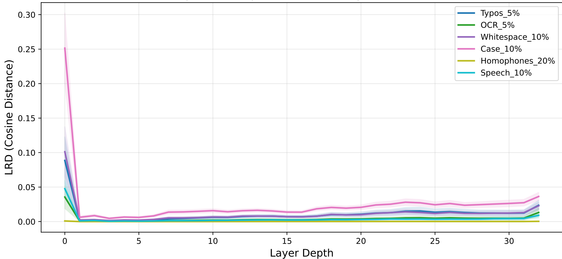
Layer-Wise Representation Divergence — BBH
