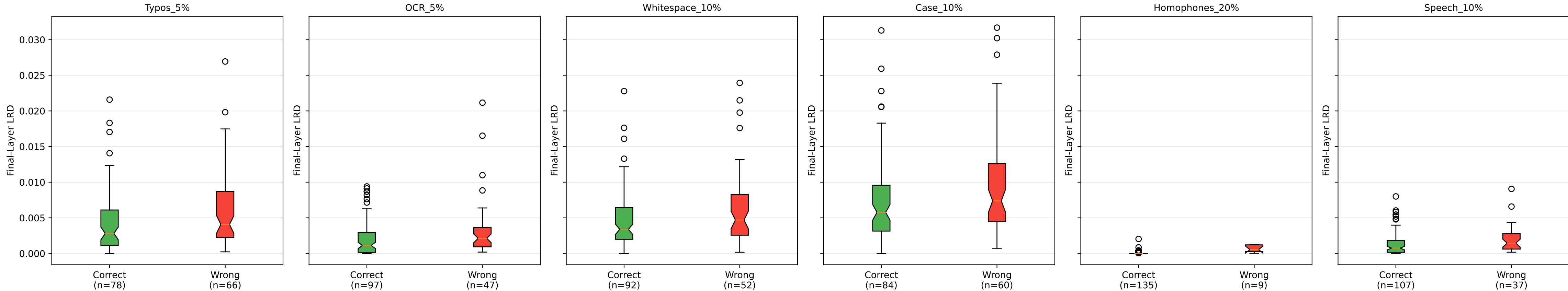
Final-Layer LRD by Task Outcome — MMLU
