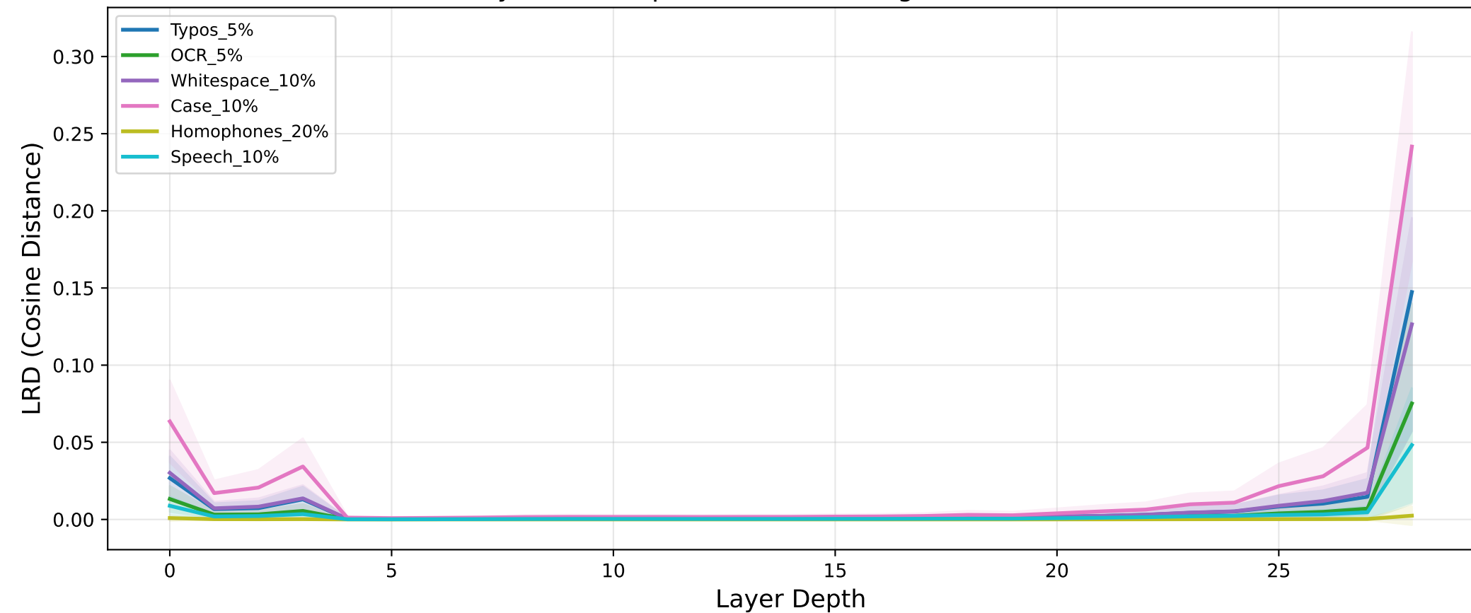
Layer-Wise Representation Divergence — GSM8K
