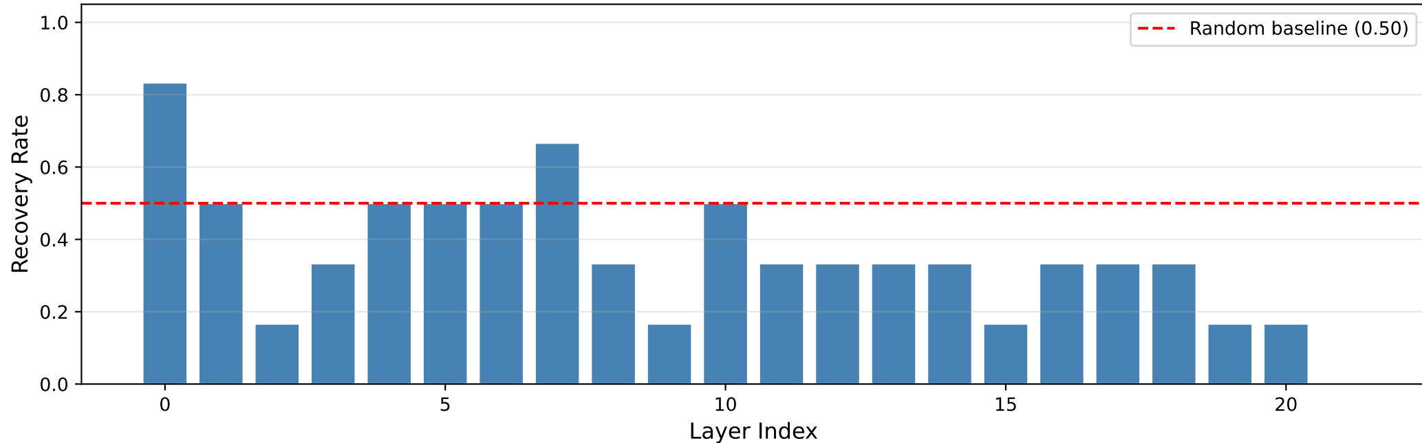
Activation Patching — GSM8K typos @ 0.05 (n=6 pairs)
