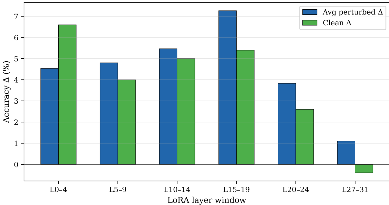
Phi-3.5: Robustness Gain by LoRA Placement
