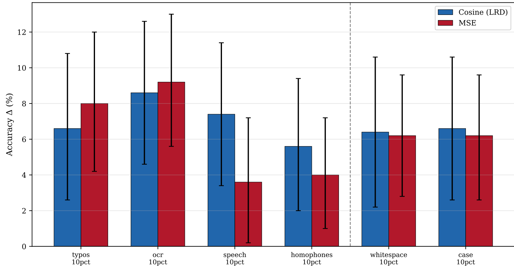
Per-Condition: Cosine vs MSE (Matched Rate 10%, L15-19, stab=24, \lambda=3.0 )
