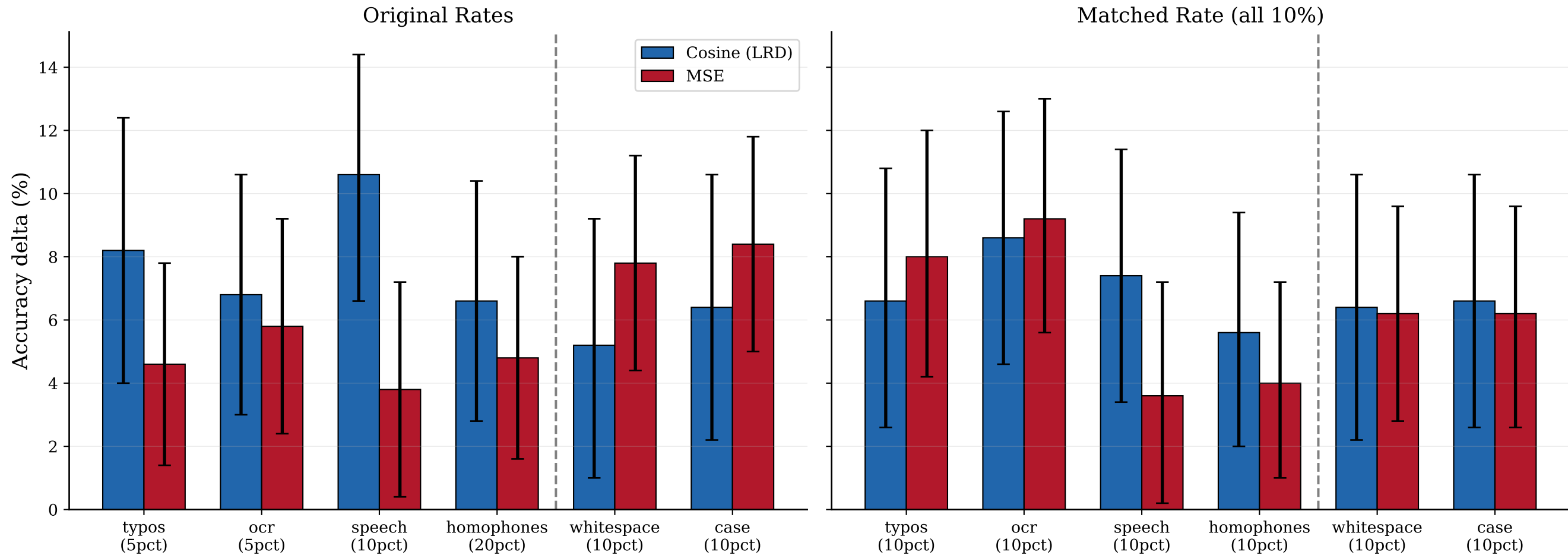
Cosine vs MSE L_{stab} : Effect of Rate Matching (Phi-3.5, L15-19, stab=24, \lambda=3.0 )
