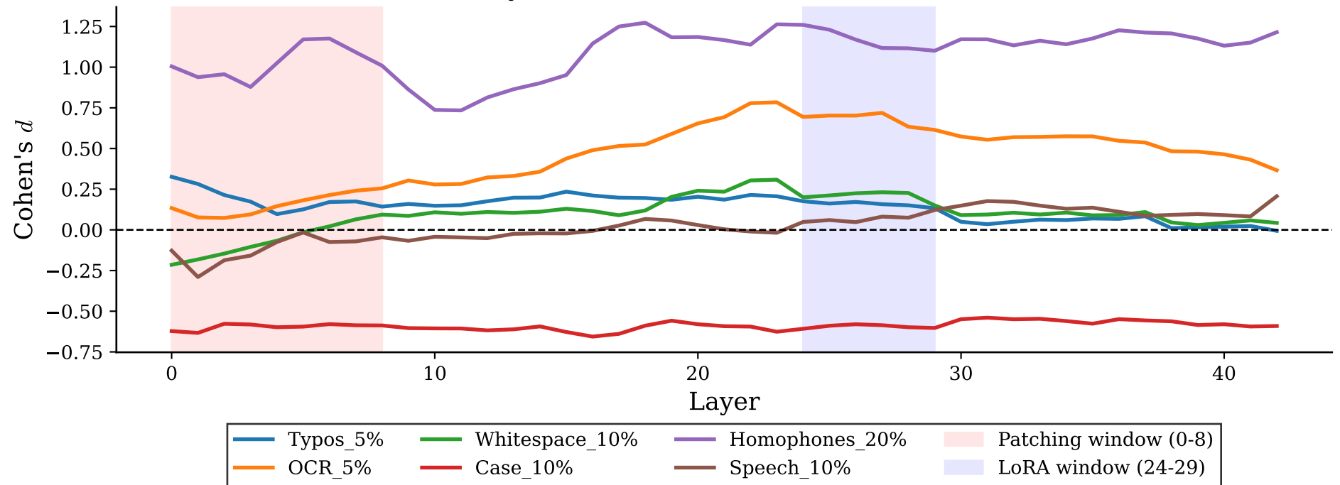
Per-Layer Cohen's d Profile - Gemma2 / GSM8K
