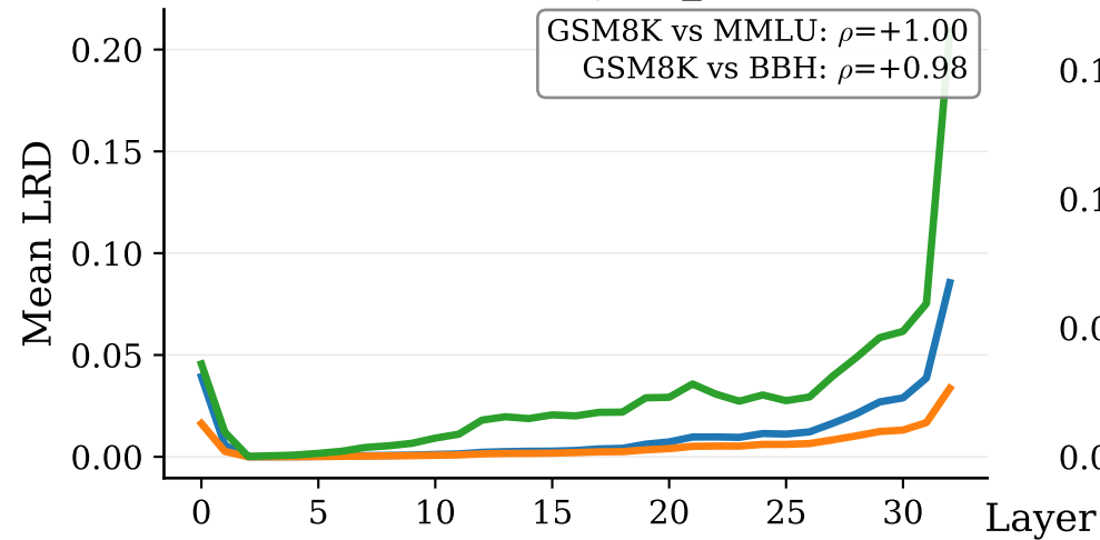
Mistral - Typos_5%
