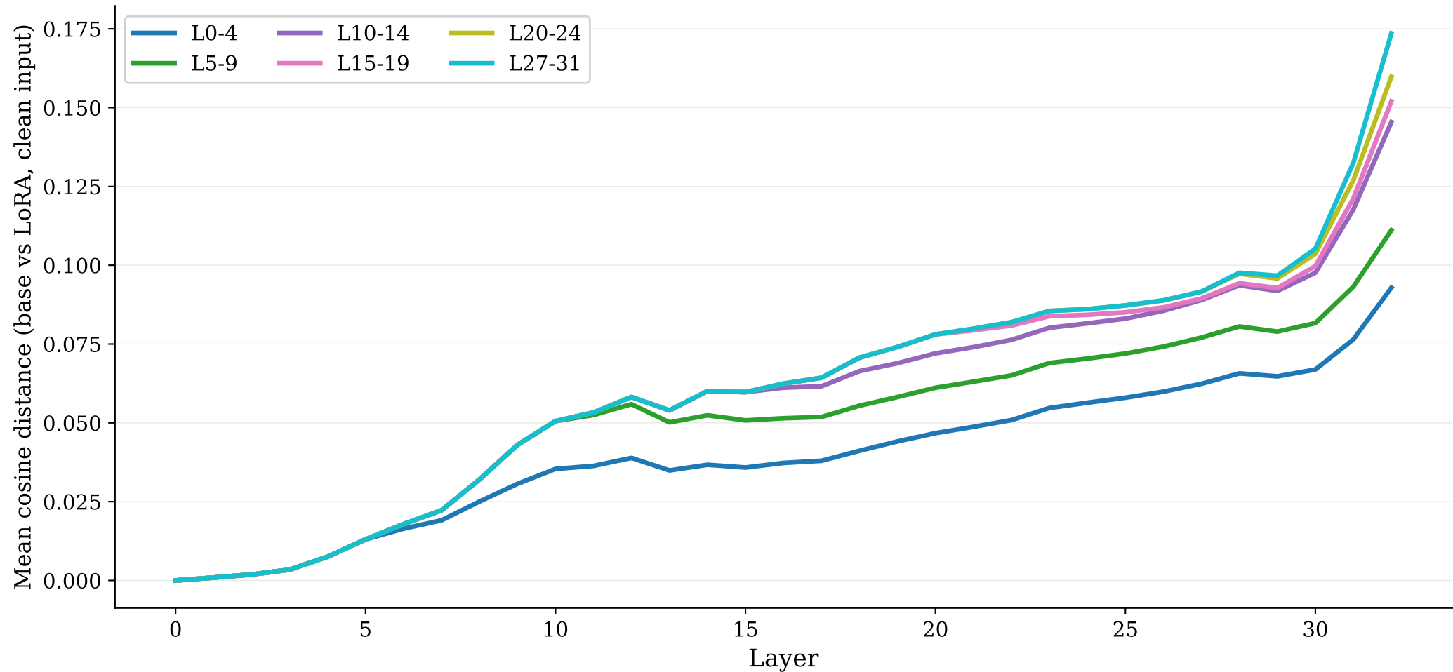
LoRA-Induced Clean Disruption - Llama-3 / GSM8K (n=200)
