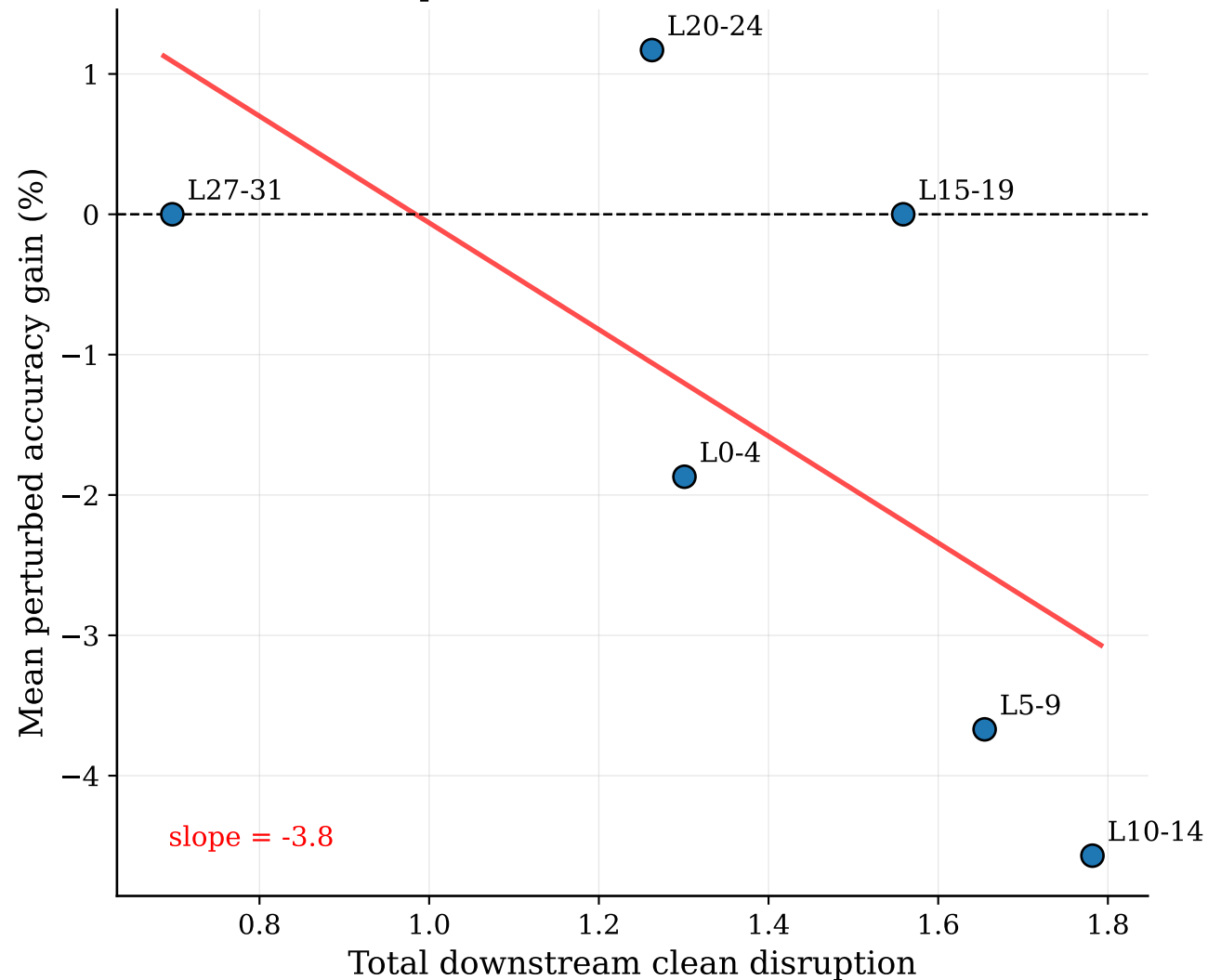
Clean Disruption vs LoRA Effectiveness - Llama-3
