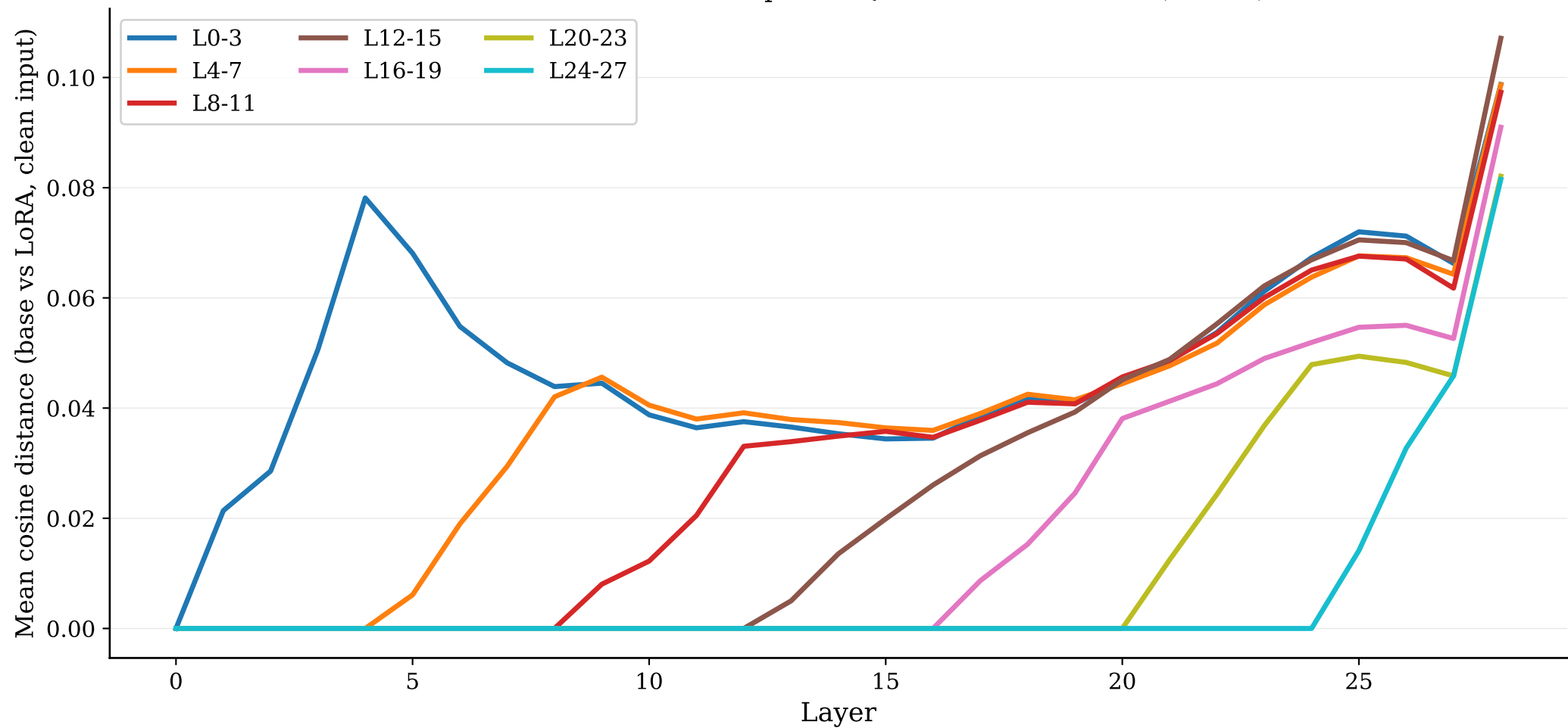
LoRA-Induced Clean Disruption - Qwen2.5-7B / GSM8K (n=200)
