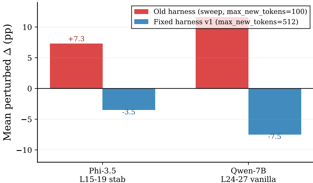
Eval-harness artifact: same checkpoint, two harnesses
