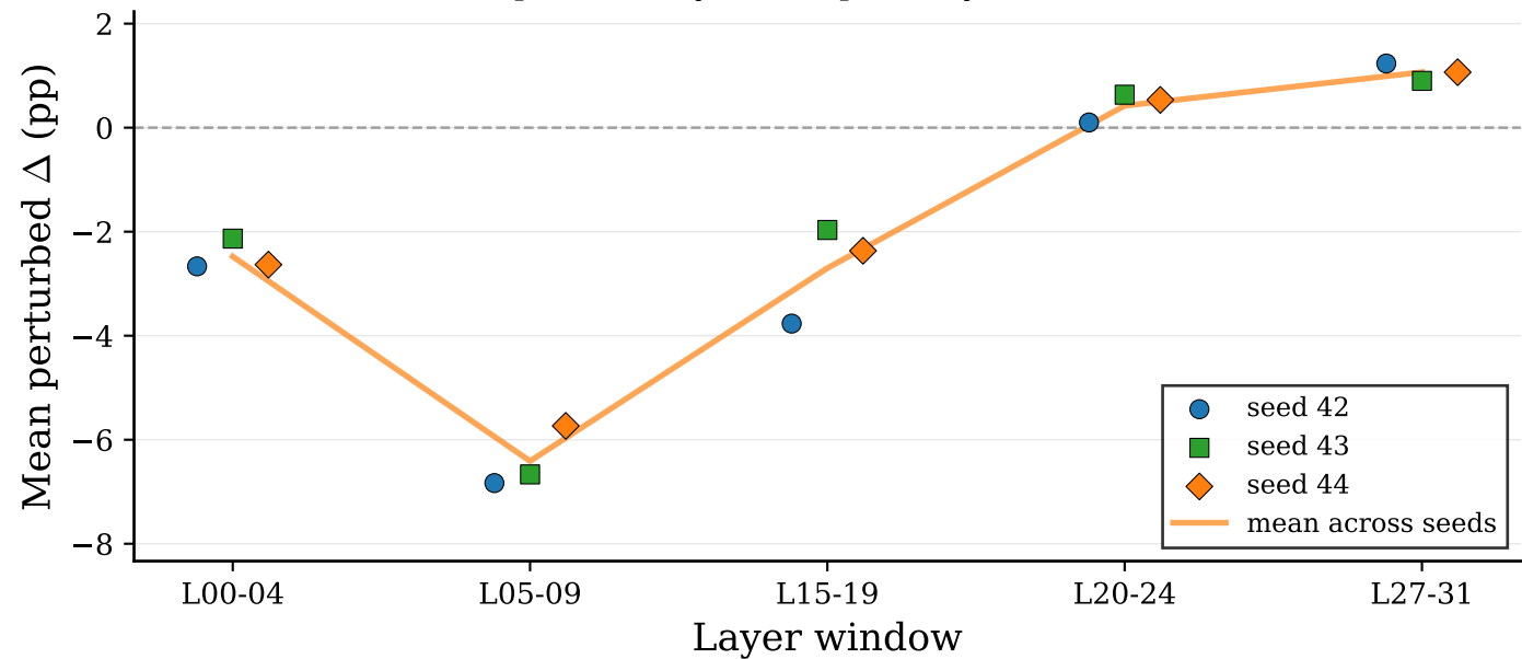
Llama-3-8B-Instruct — per-seed layer sweep (32 layers)
