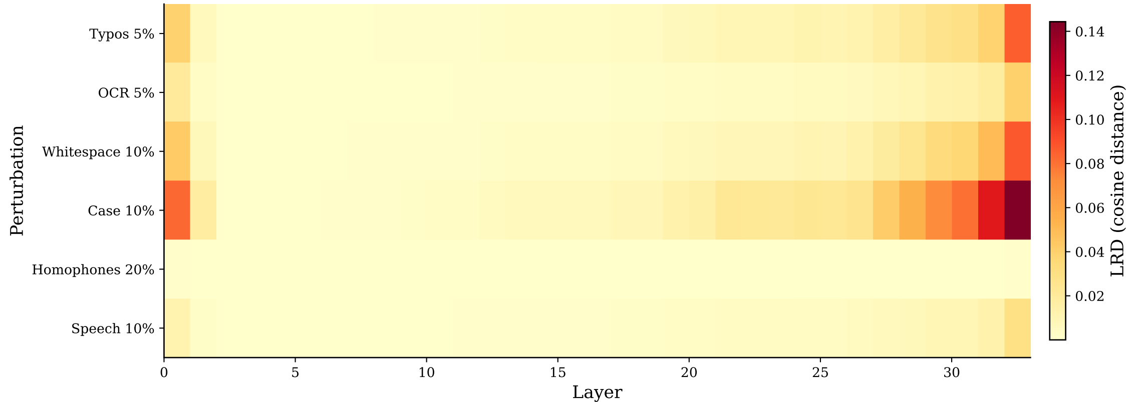
LRD Heatmap (mean across examples)
