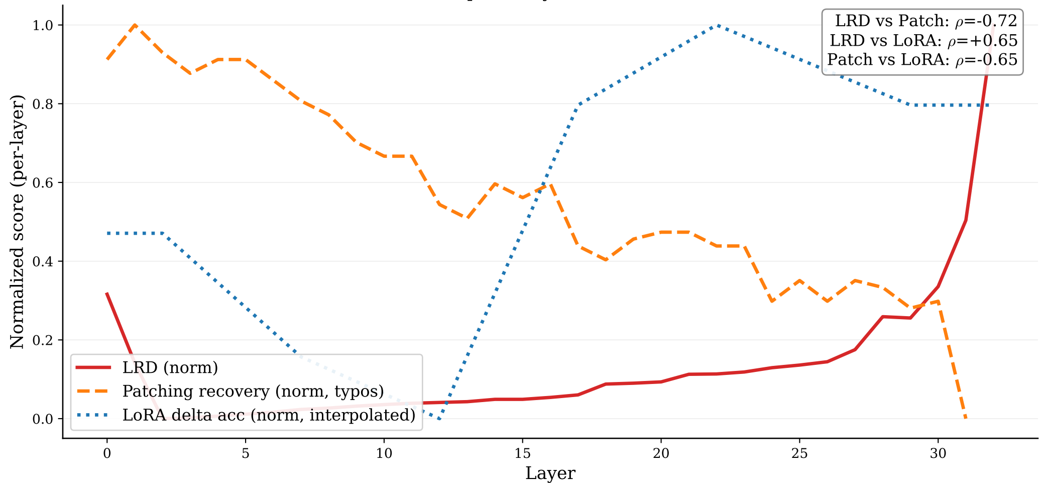
Three-Map Overlay - Llama3 / GSM8K
