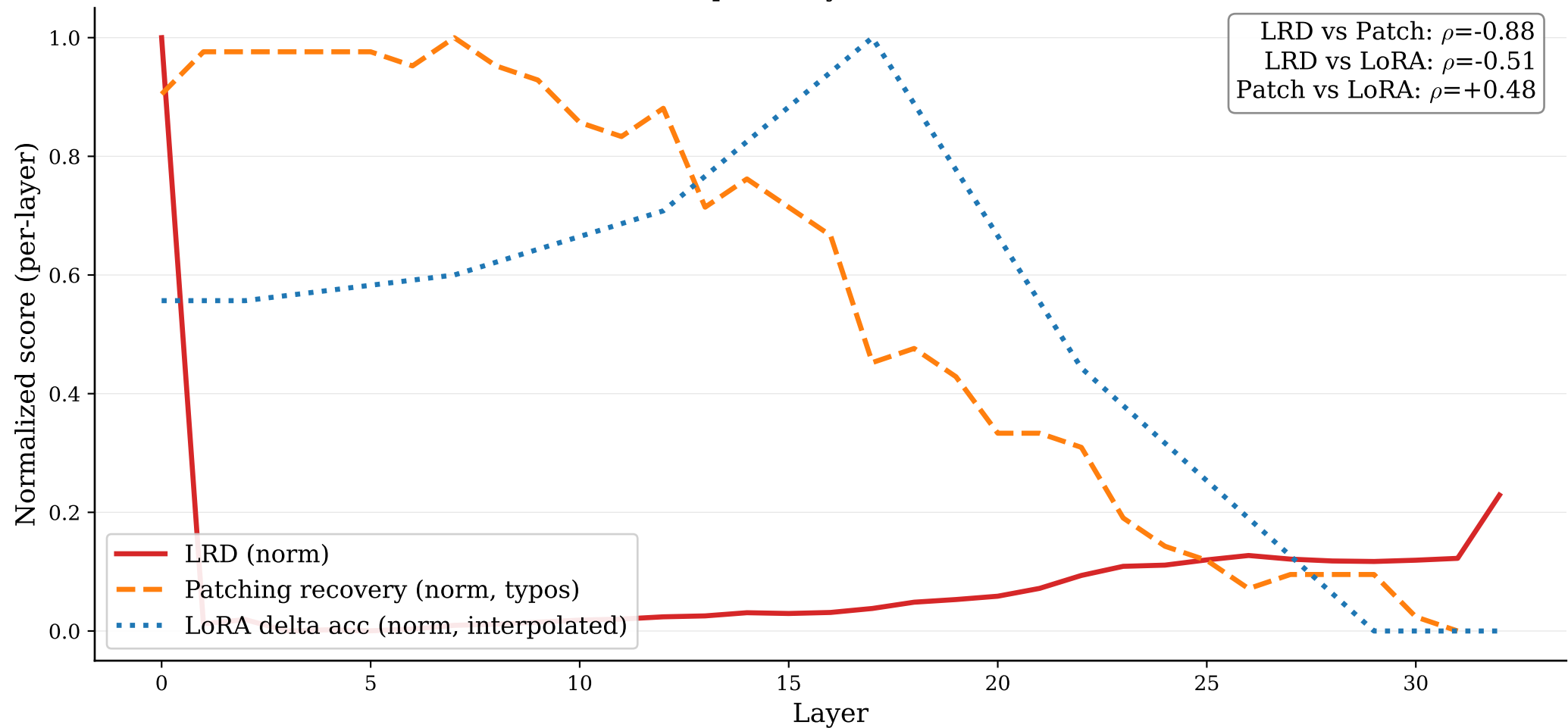
Three-Map Overlay - Phi3.5 / GSM8K
