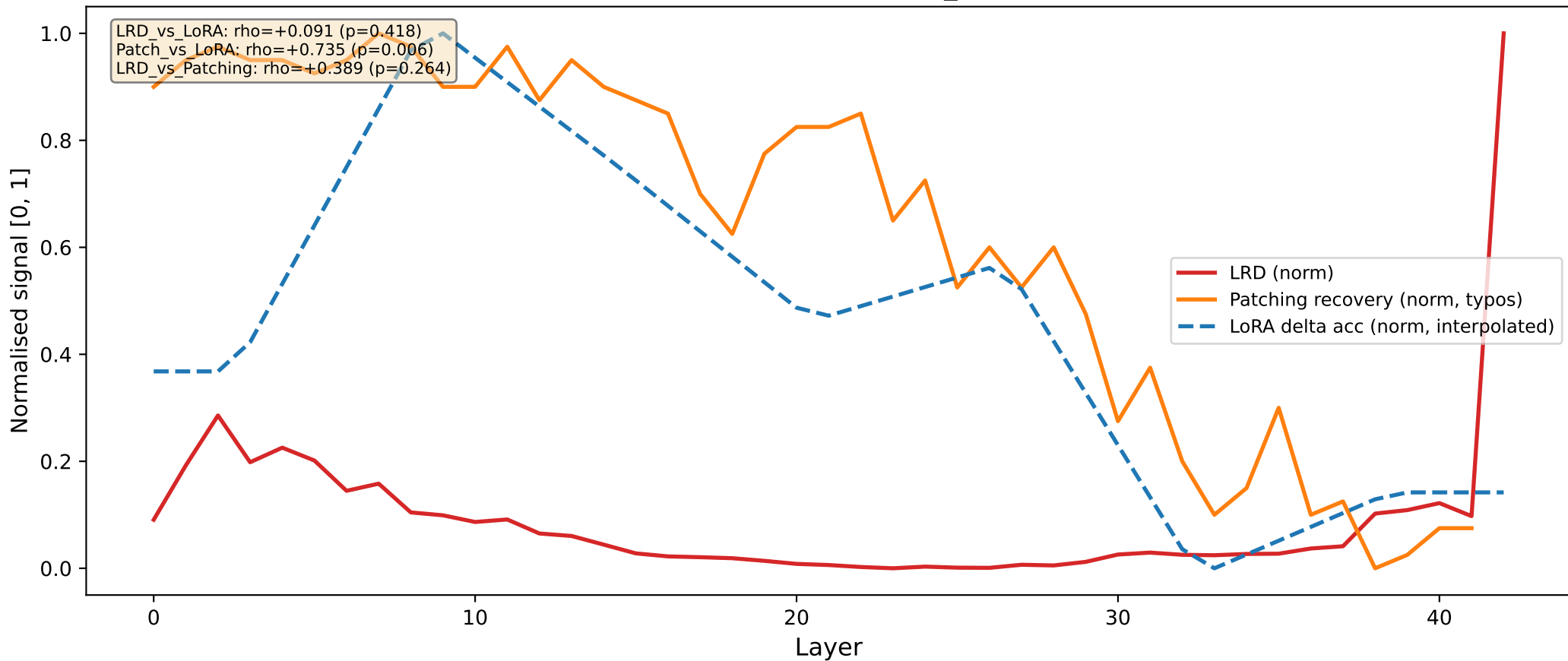
Three-Map Overlay - Gemma2_9B / GSM8K
