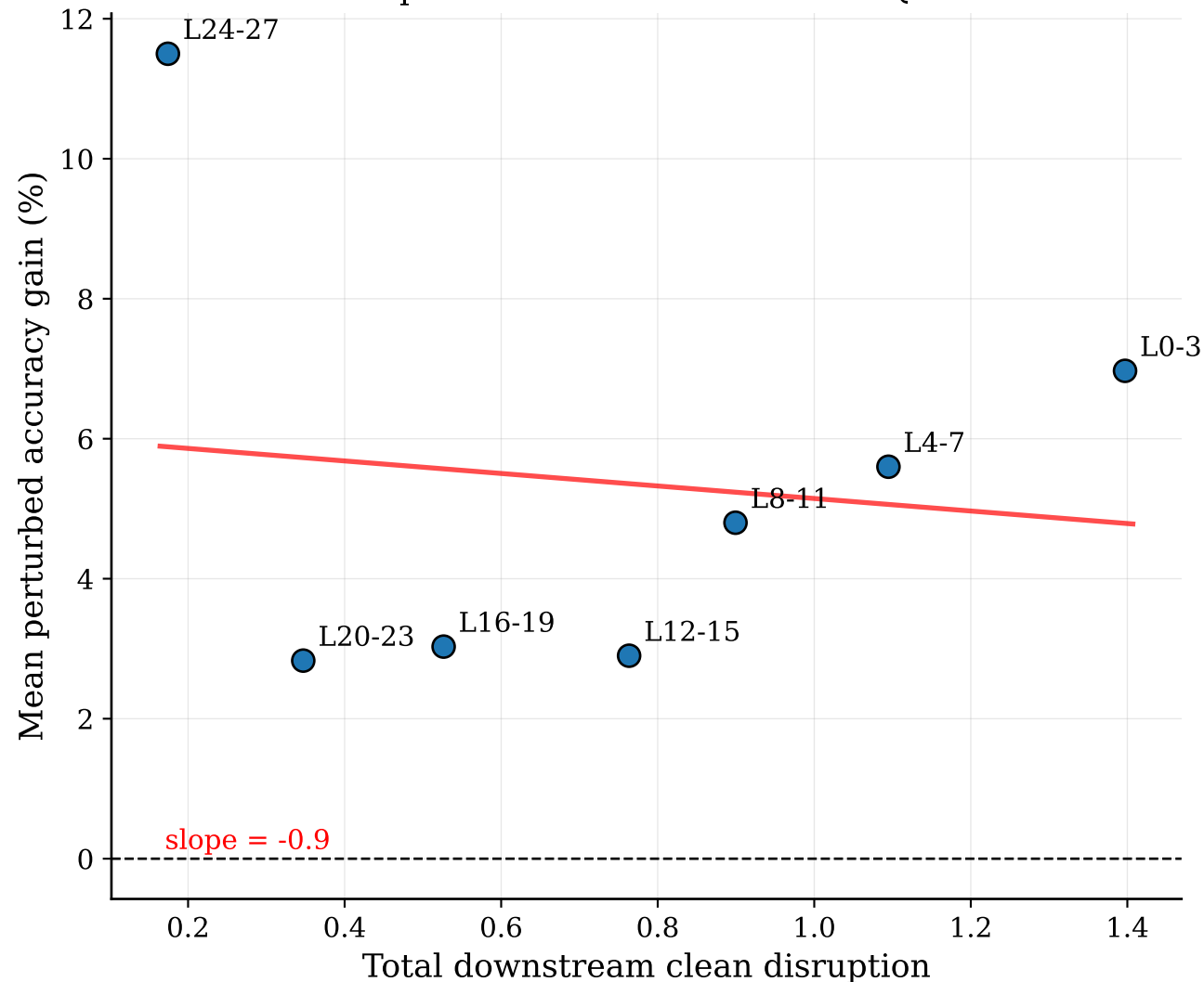
Clean Disruption vs LoRA Effectiveness - Qwen2.5-7B
