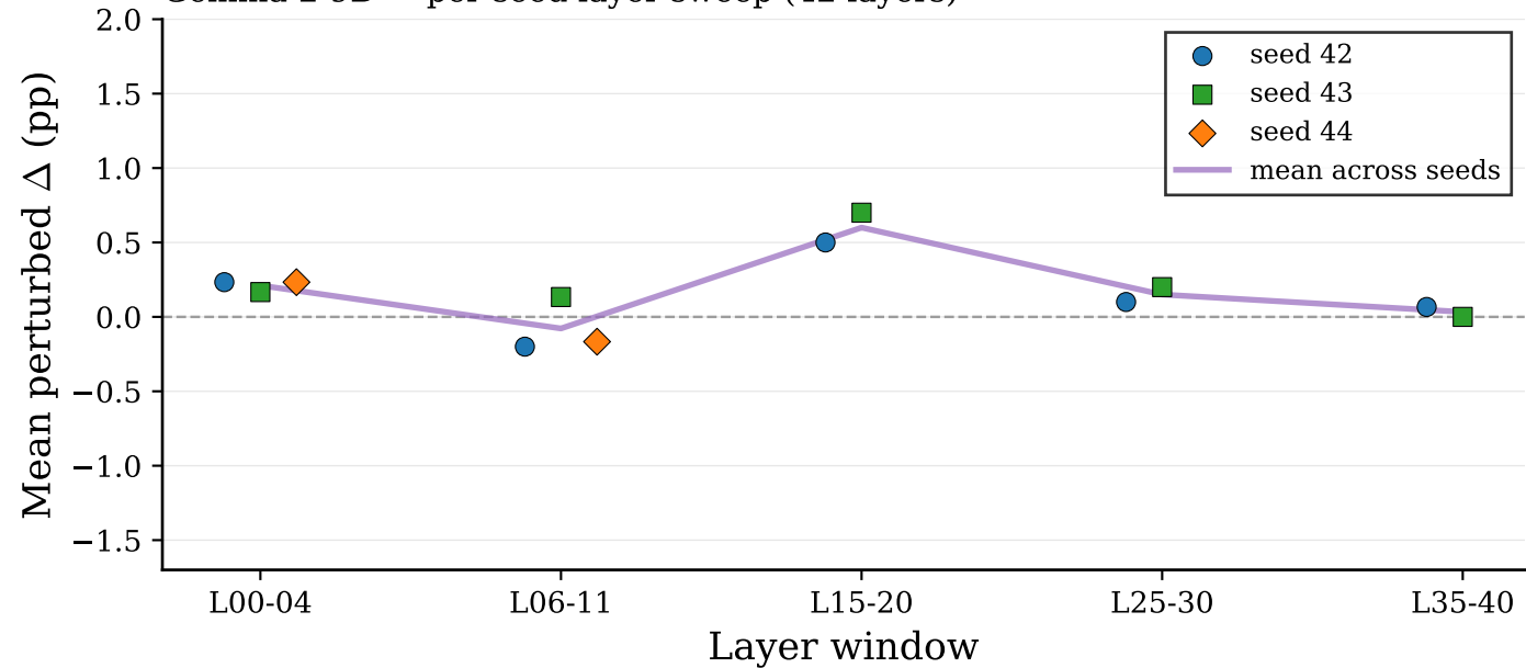
Gemma-2-9B — per-seed layer sweep (42 layers)
