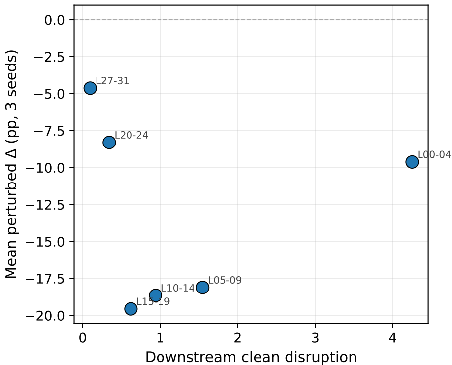
Mistral-7B-v0.3 (retrained adapters) Spearman \rho = -0.429
