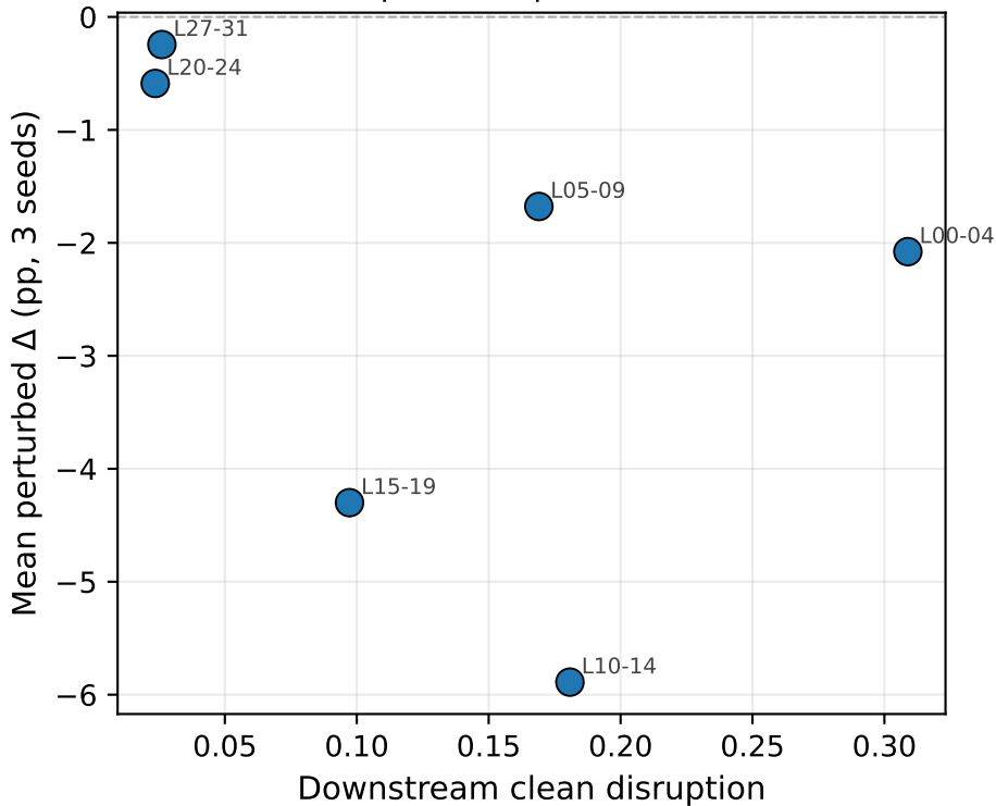
Phi-3.5-mini (retrained adapters) Spearman \rho = -0.657
