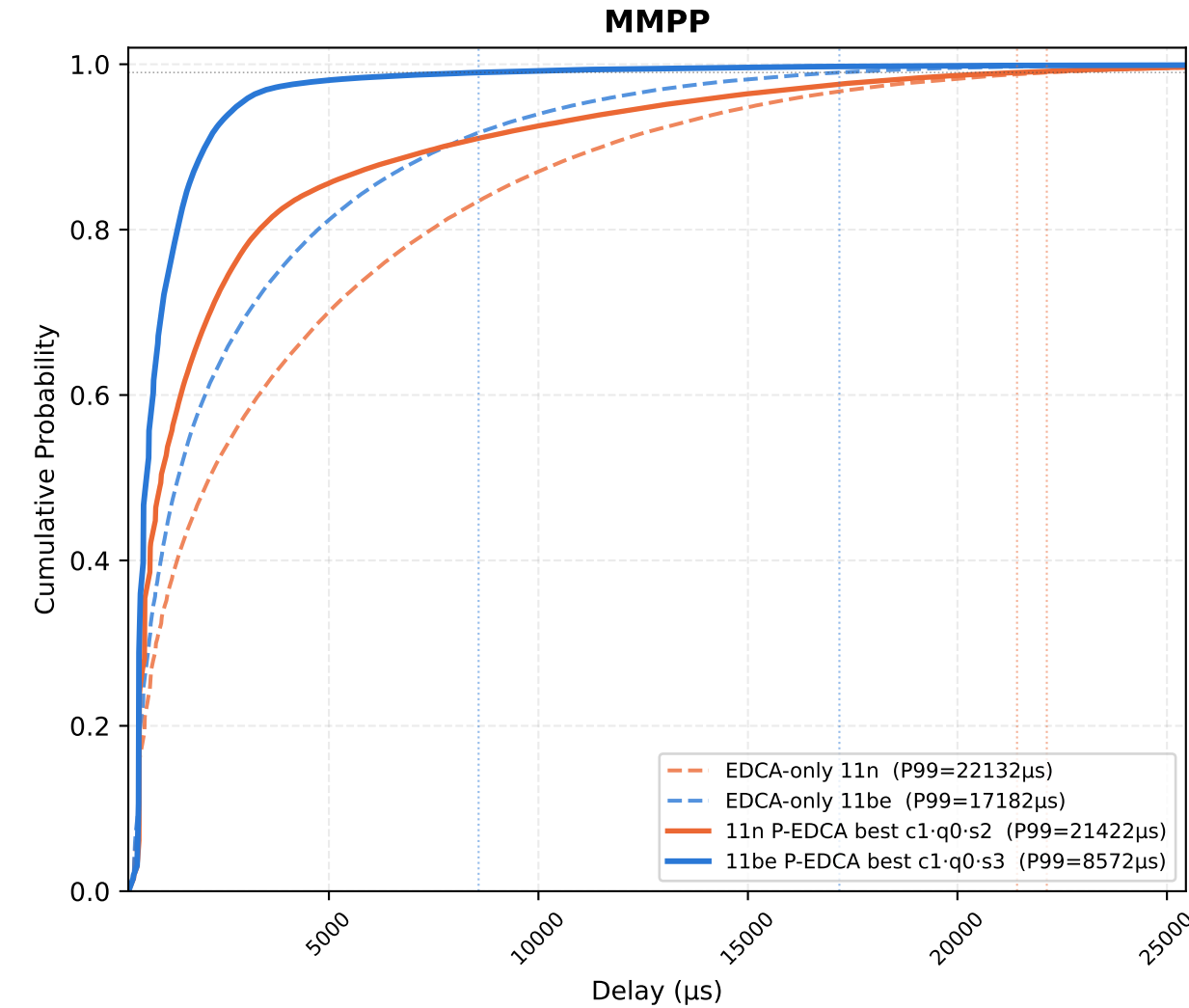
All STAs — EDCA-only (11n / 11be) vs Best-param P-EDCA (11n / 11be) | nPedca=30/30, nSta=30, 1Mbps, 10 runs avg
