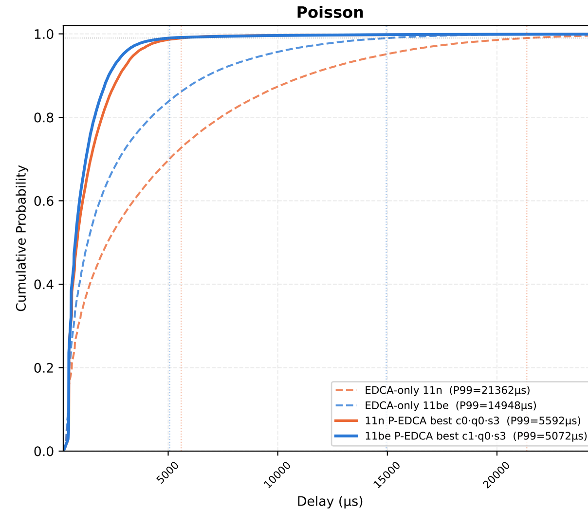
P-EDCA STAs — EDCA-only (11n / 11be) vs Best-param P-EDCA (11n / 11be) | nPedca=5/30, nSta=30, 1Mbps, 10 runs avg
