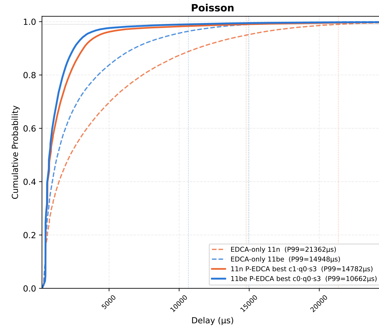
P-EDCA STAs — EDCA-only (11n / 11be) vs Best-param P-EDCA (11n / 11be) | nPedca=15/30, nSta=30, 1Mbps, 10 runs avg
