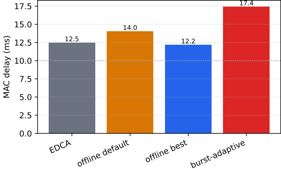
nPEDCA=30: loss-aware R(10 ms)
