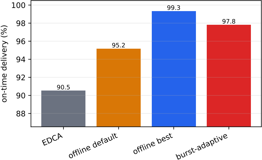
nPEDCA=5: loss-aware R(10 ms)
