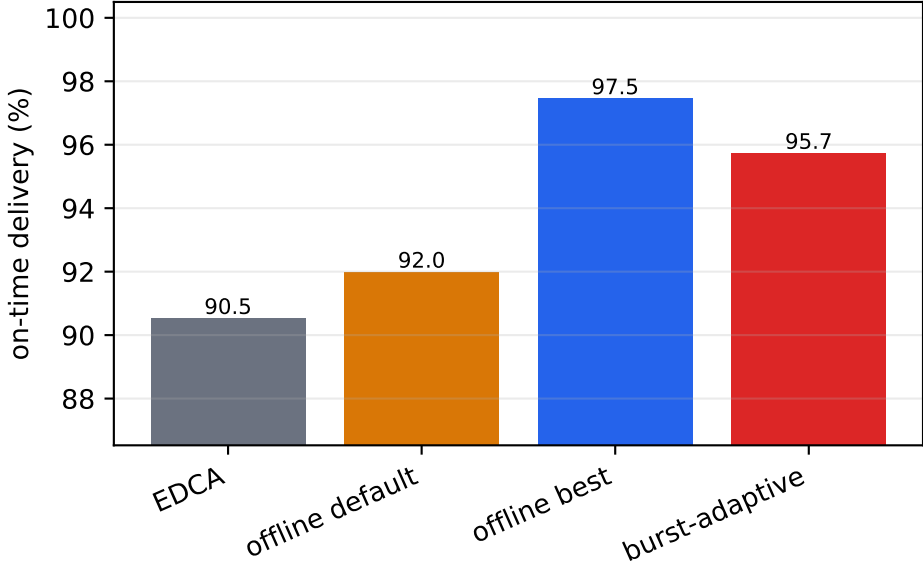
nPEDCA=15: loss-aware R(10 ms)
