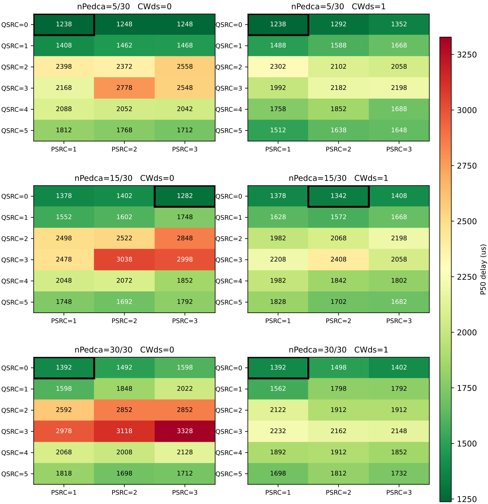
P-EDCA STA VO Delay — Median Dual-DS (2x DS-CTS) (nSta=30, 1Mbps, black box = best in panel) colour scale 1238-3328 shared across mono-DS & dual-DS — panels are directly comparable
