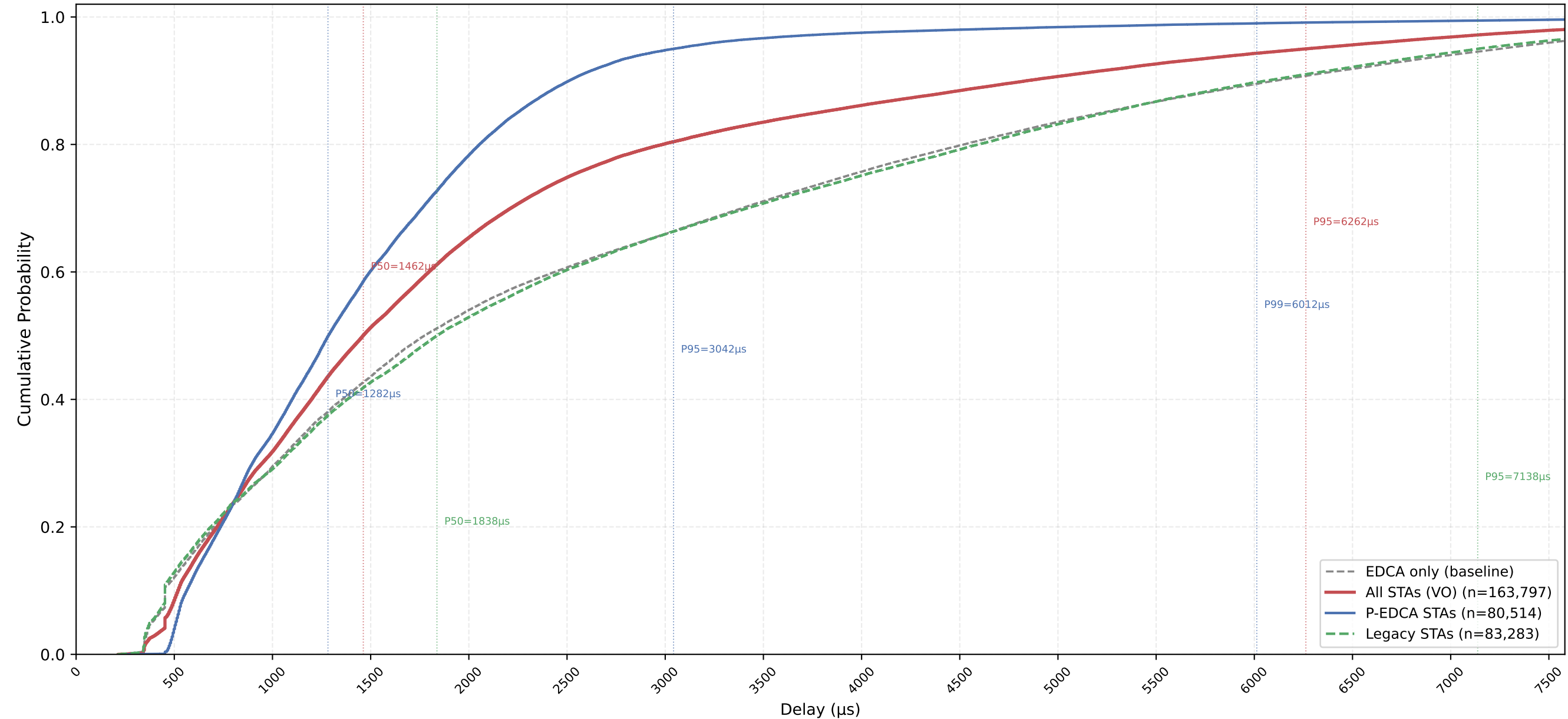
VO Delay CDF — P-EDCA / Legacy / All | CWds=0 × QSRC=0 × PSRC=3 nSta=30, nPedca=15/30, 1Mbps, avg of 10 runs
