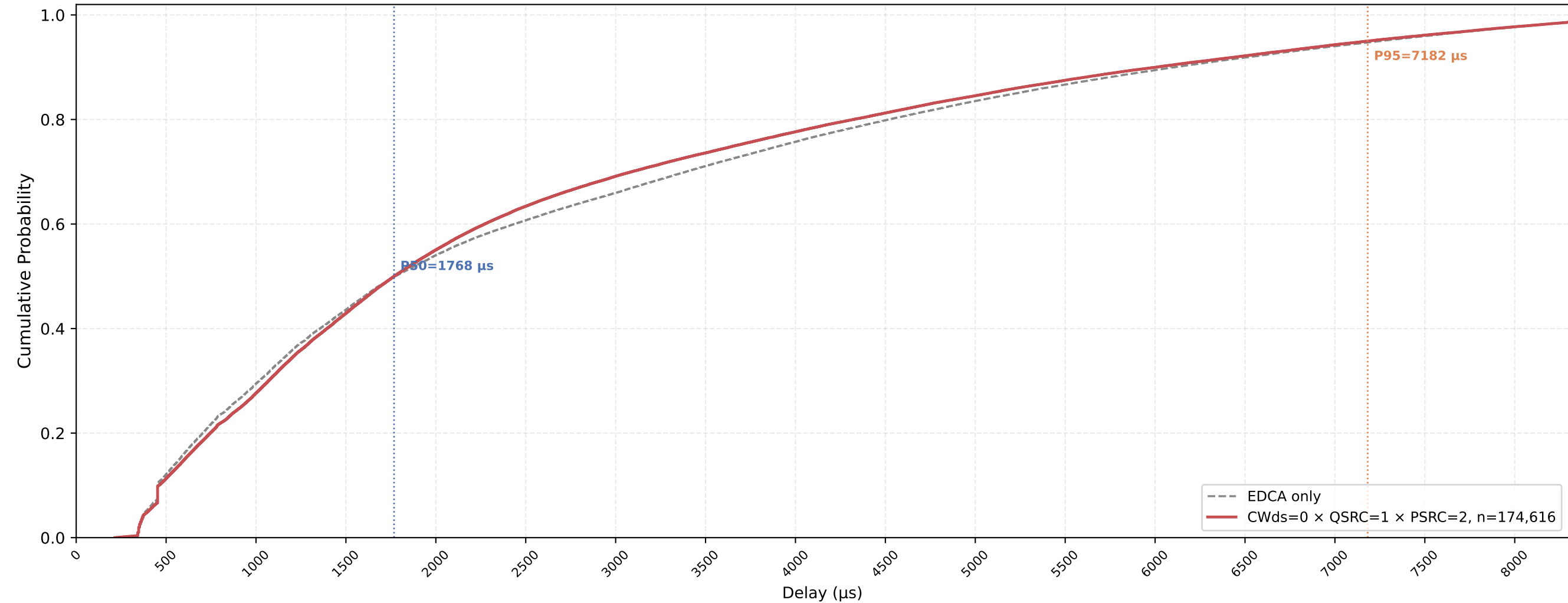
VO (all STAs) Delay CDF — CWds=0 × QSRC=1 × PSRC=2 nSta=30, nPedca=5, 1Mbps, avg of 10 runs
